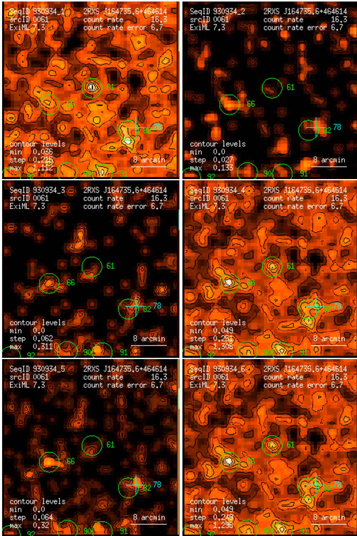
Figure 61: RASS 930934: detection 0061: band rate images, Gaussian filter: (1) PSPC channels 11 – 41, (2) 52 – 90, (3) 91 – 201, (4) 11 – 235, (5) 52 – 201, (6) 11 – 201. Broad band rates in counts/ks. Band rate contour levels in counts/ks/arcmin 2 .
