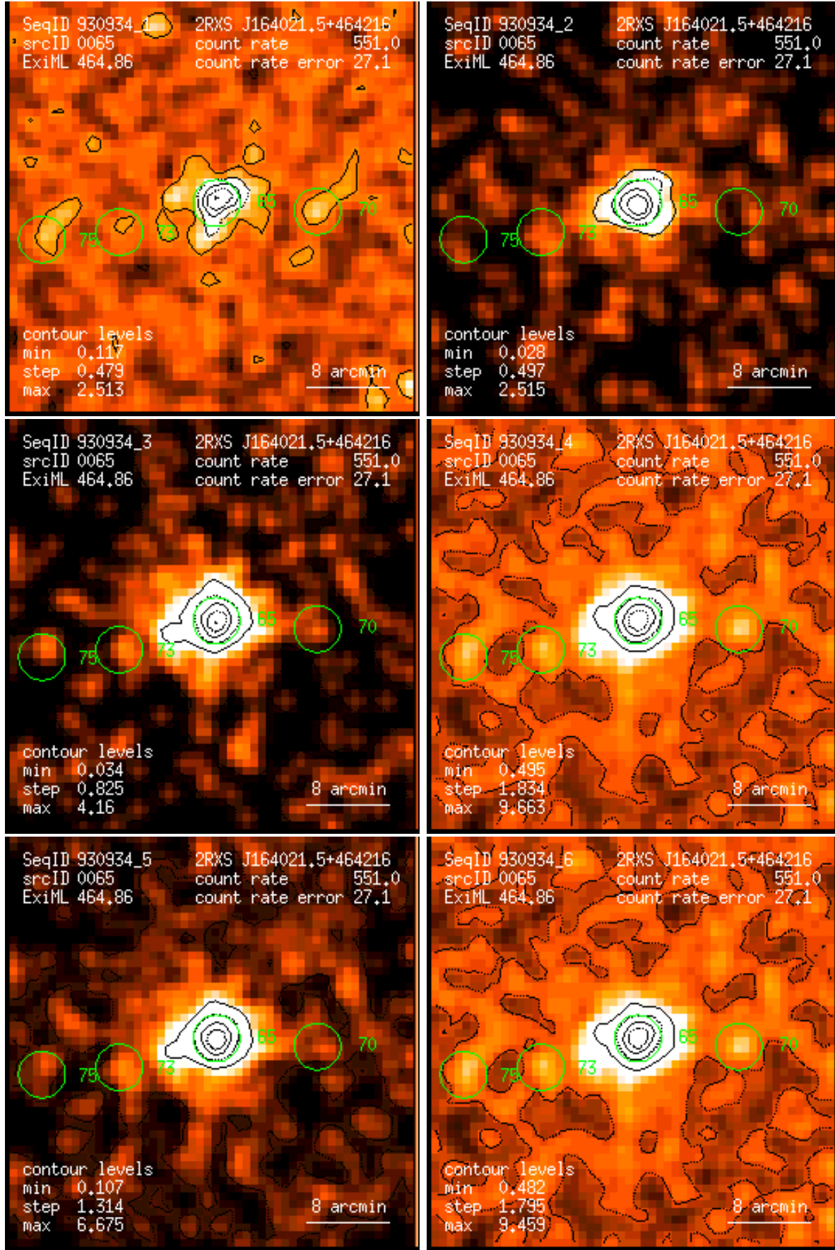
Figure 65: RASS 930934: detection 0065: band rate images, Gaussian filter: (1) PSPC channels 11 – 41, (2) 52 – 90, (3) 91 – 201, (4) 11 – 235, (5) 52 – 201, (6) 11 – 201. Broad band rates in counts/ks. Band rate contour levels in counts/ks/arcmin 2 .
