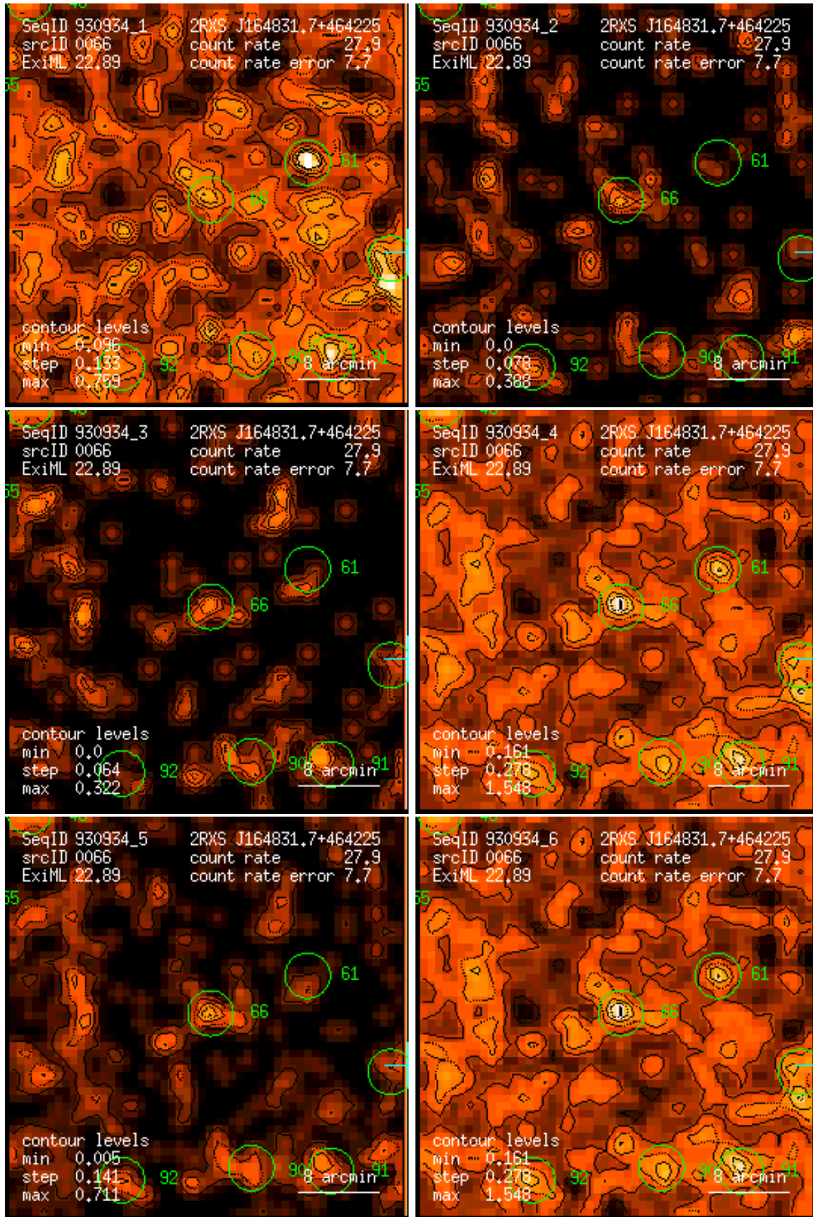
Figure 66: RASS 930934: detection 0066: band rate images, Gaussian filter: (1) PSPC channels 11 – 41, (2) 52 – 90, (3) 91 – 201, (4) 11 – 235, (5) 52 – 201, (6) 11 – 201. Broad band rates in counts/ks. Band rate contour levels in counts/ks/arcmin 2 .
