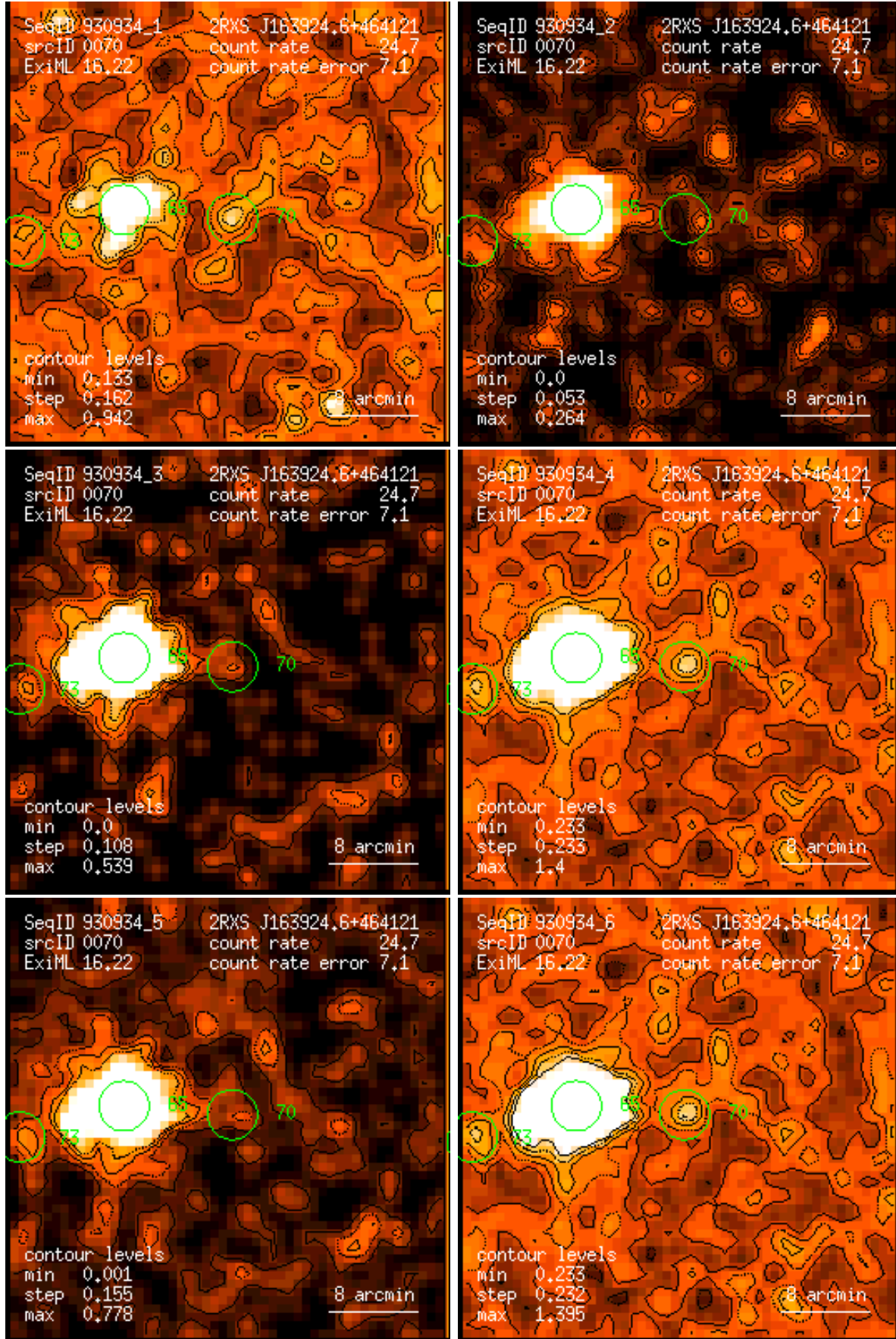
Figure 70: RASS 930934: detection 0070: band rate images, Gaussian filter: (1) PSPC channels 11 – 41, (2) 52 – 90, (3) 91 – 201, (4) 11 – 235, (5) 52 – 201, (6) 11 – 201. Broad band rates in counts/ks. Band rate contour levels in counts/ks/arcmin 2 .
