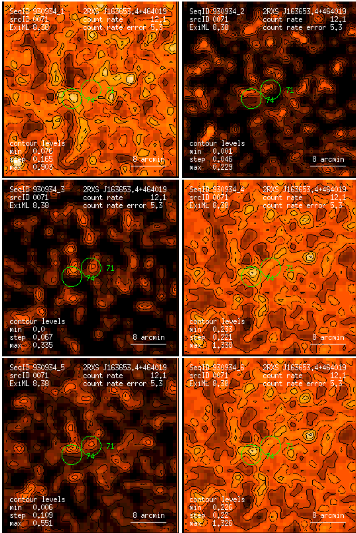
Figure 71: RASS 930934: detection 0071: band rate images, Gaussian filter: (1) PSPC channels 11 – 41, (2) 52 – 90, (3) 91 – 201, (4) 11 – 235, (5) 52 – 201, (6) 11 – 201. Broad band rates in counts/ks. Band rate contour levels in counts/ks/arcmin 2 .
