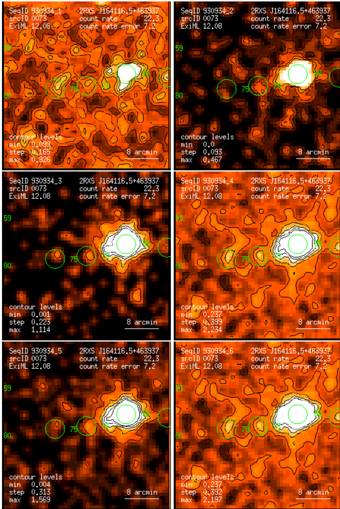
Figure 73: RASS 930934: detection 0073: band rate images, Gaussian filter: (1) PSPC channels 11 – 41, (2) 52 – 90, (3) 91 – 201, (4) 11 – 235, (5) 52 – 201, (6) 11 – 201. Broad band rates in counts/ks. Band rate contour levels in counts/ks/arcmin 2 .
