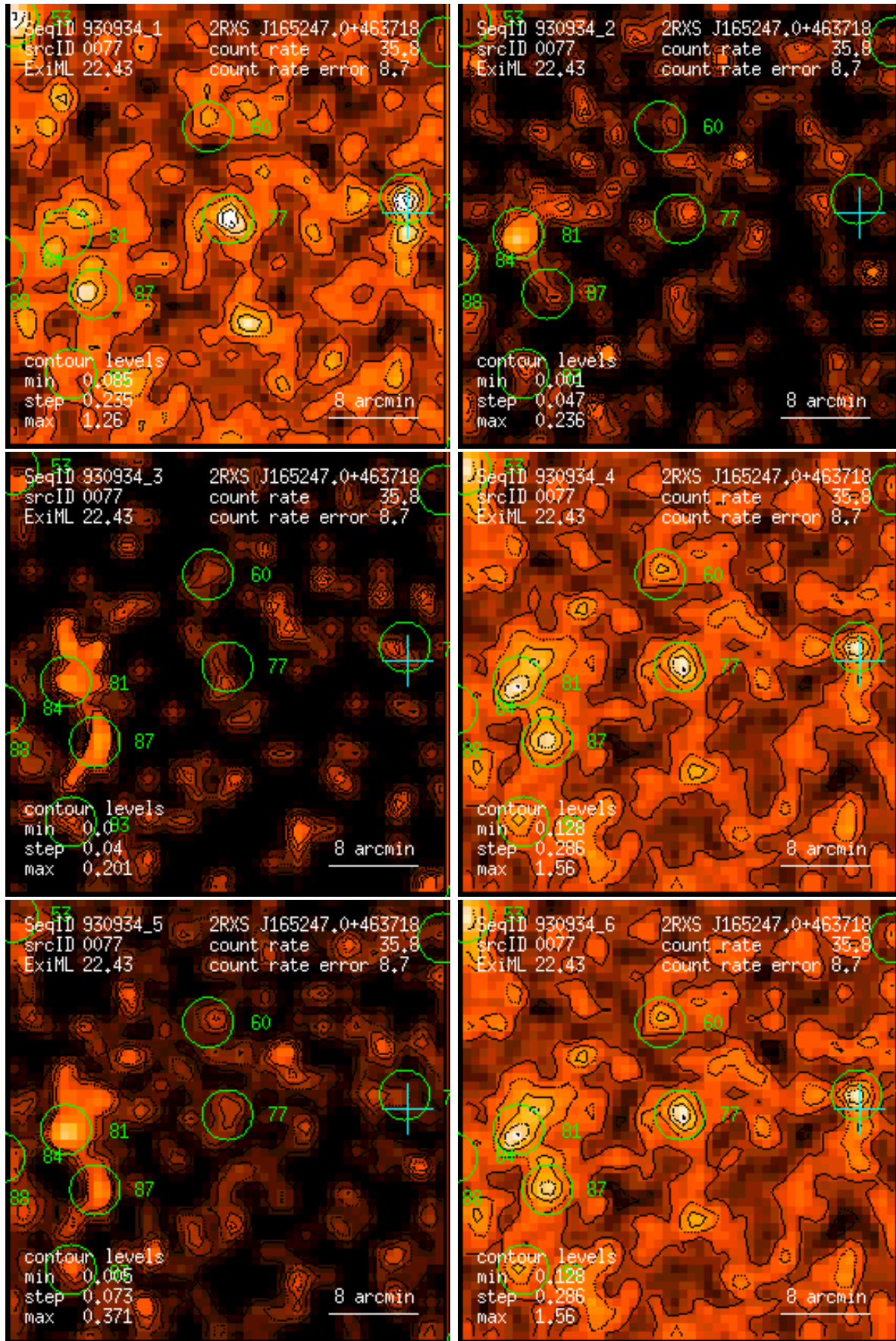
Figure 77: RASS 930934: detection 0077: band rate images, Gaussian filter: (1) PSPC channels 11 – 41, (2) 52 – 90, (3) 91 – 201, (4) 11 – 235, (5) 52 – 201, (6) 11 – 201. Broad band rates in counts/ks. Band rate contour levels in counts/ks/arcmin 2 .
