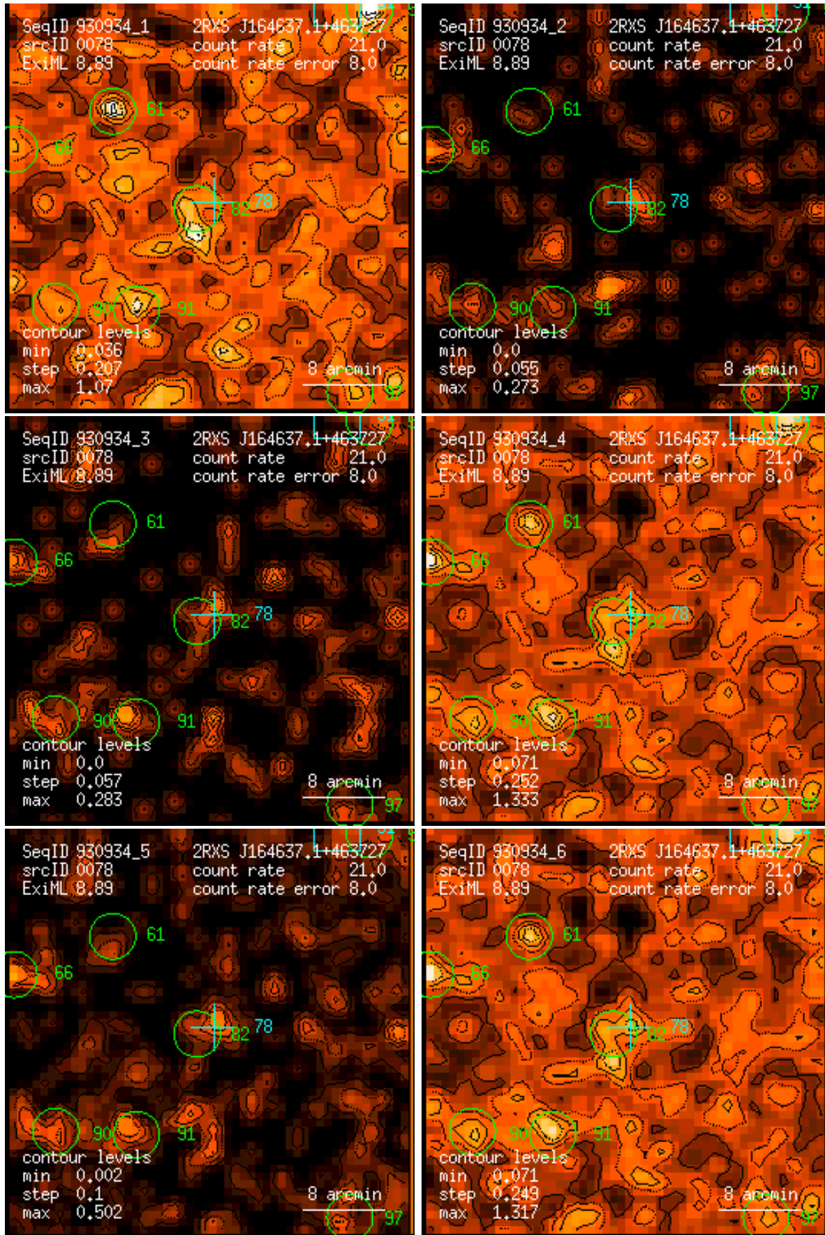
Figure 78: RASS 930934: detection 0078: band rate images, Gaussian filter: (1) PSPC channels 11 – 41, (2) 52 – 90, (3) 91 – 201, (4) 11 – 235, (5) 52 – 201, (6) 11 – 201. Broad band rates in counts/ks. Band rate contour levels in counts/ks/arcmin 2 .
