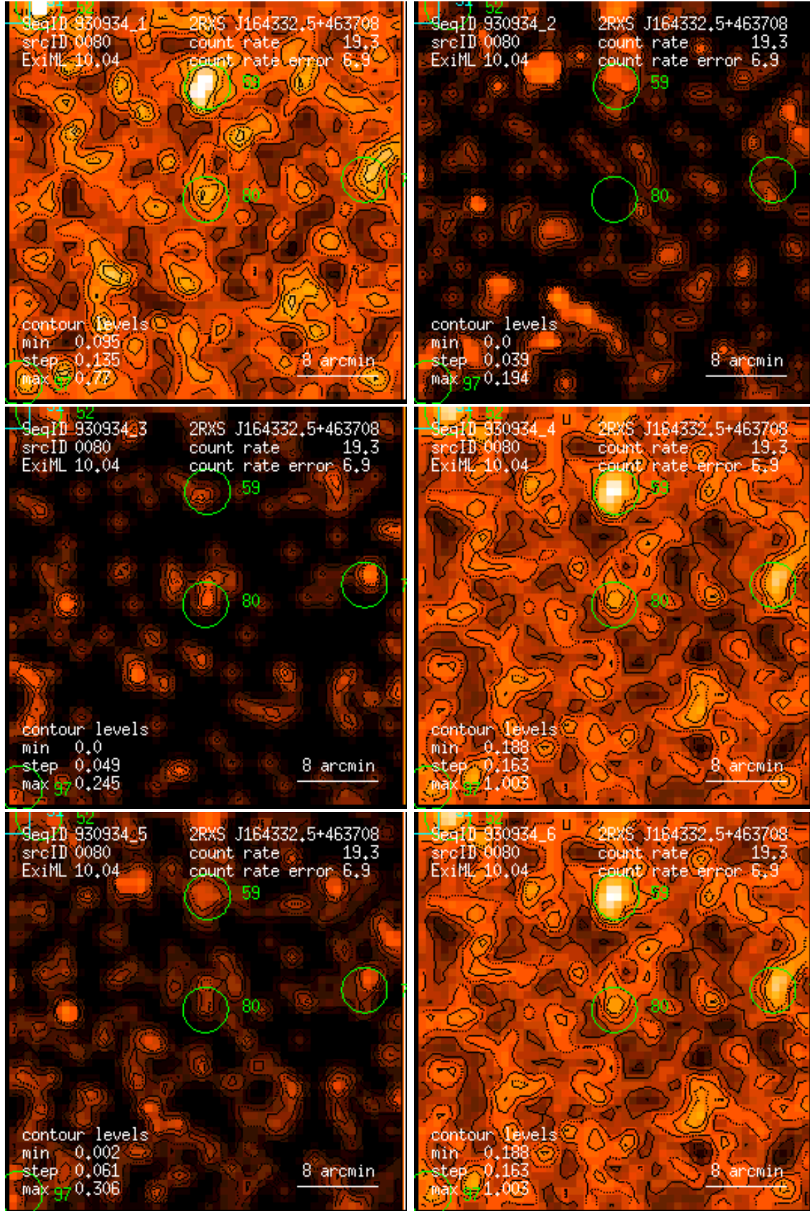
Figure 80: RASS 930934: detection 0080: band rate images, Gaussian filter: (1) PSPC channels 11 – 41, (2) 52 – 90, (3) 91 – 201, (4) 11 – 235, (5) 52 – 201, (6) 11 – 201. Broad band rates in counts/ks. Band rate contour levels in counts/ks/arcmin 2 .
