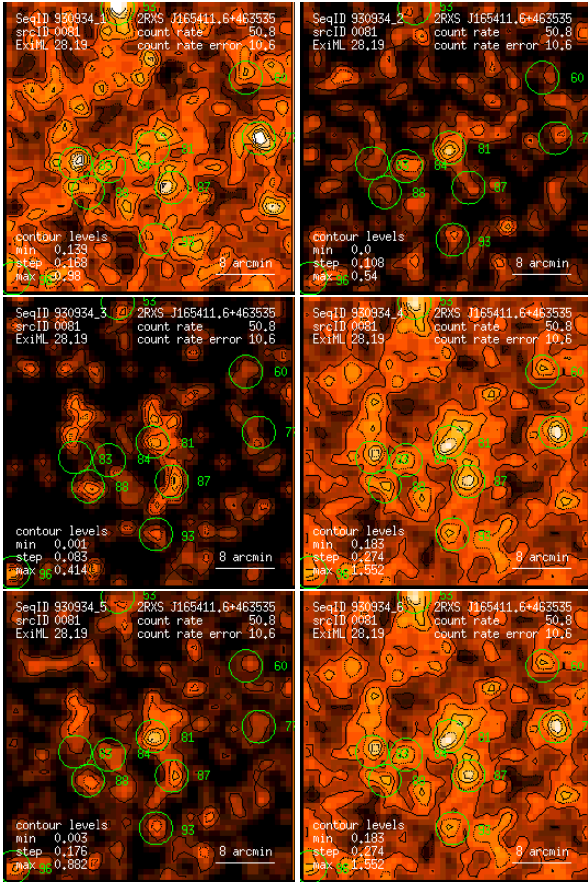
Figure 81: RASS 930934: detection 0081: band rate images, Gaussian filter: (1) PSPC channels 11 – 41, (2) 52 – 90, (3) 91 – 201, (4) 11 – 235, (5) 52 – 201, (6) 11 – 201. Broad band rates in counts/ks. Band rate contour levels in counts/ks/arcmin 2 .
