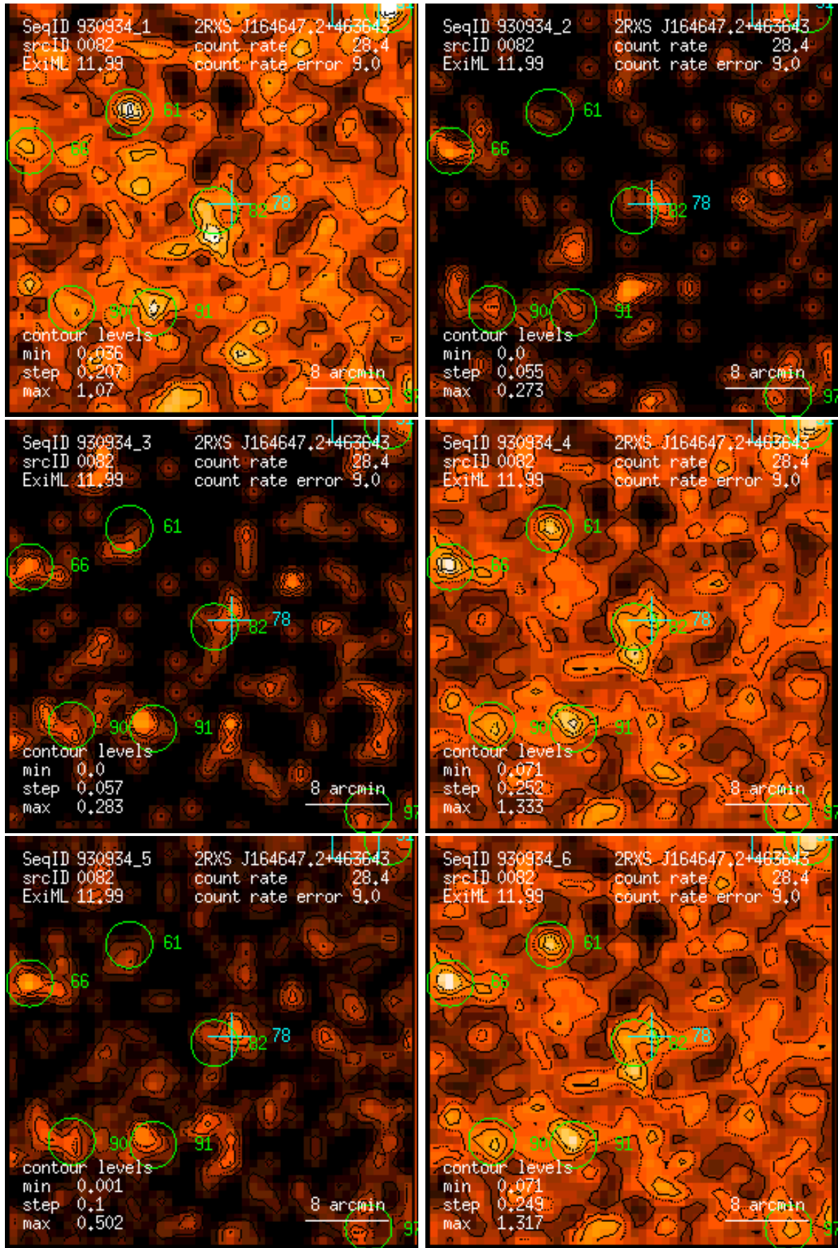
Figure 82: RASS 930934: detection 0082: band rate images, Gaussian filter: (1) PSPC channels 11 – 41, (2) 52 – 90, (3) 91 – 201, (4) 11 – 235, (5) 52 – 201, (6) 11 – 201. Broad band rates in counts/ks. Band rate contour levels in counts/ks/arcmin 2 .
