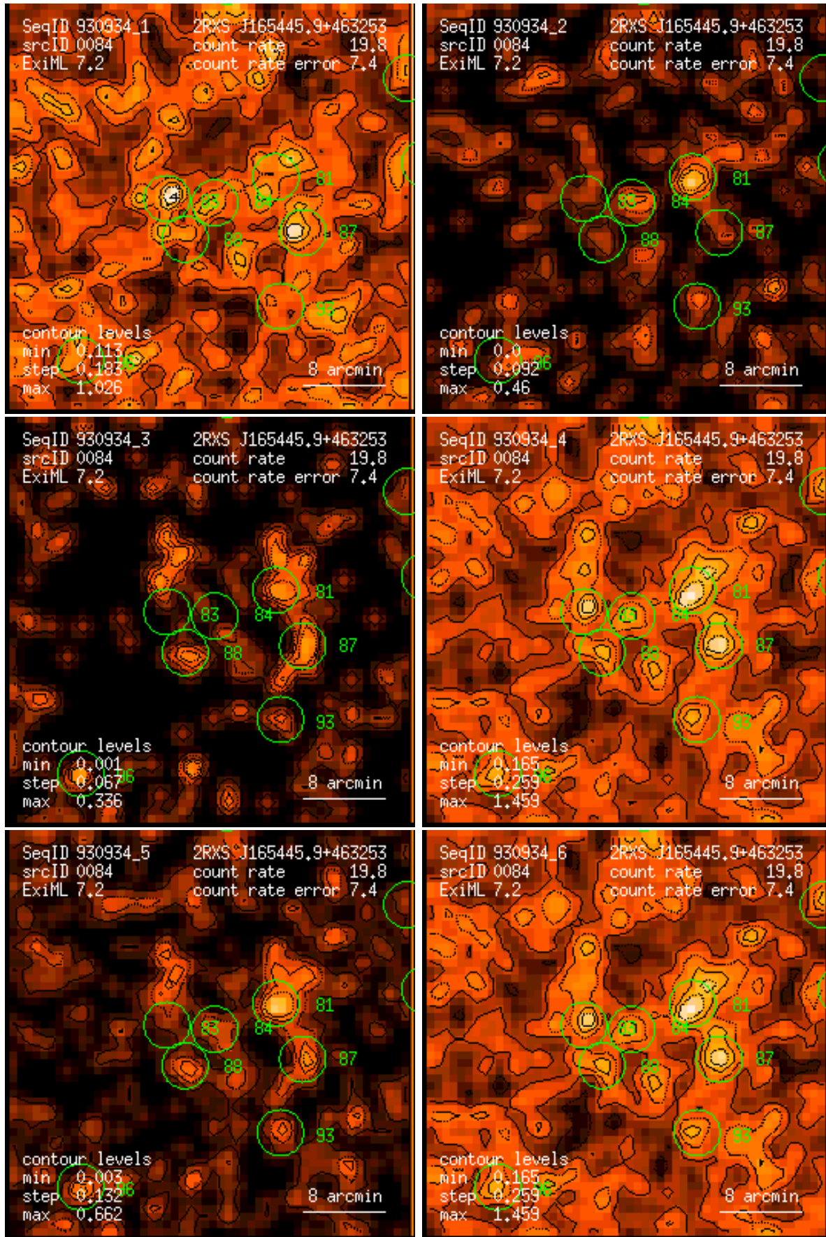
Figure 84: RASS 930934: detection 0084: band rate images, Gaussian filter: (1) PSPC channels 11 – 41, (2) 52 – 90, (3) 91 – 201, (4) 11 – 235, (5) 52 – 201, (6) 11 – 201. Broad band rates in counts/ks. Band rate contour levels in counts/ks/arcmin 2 .
