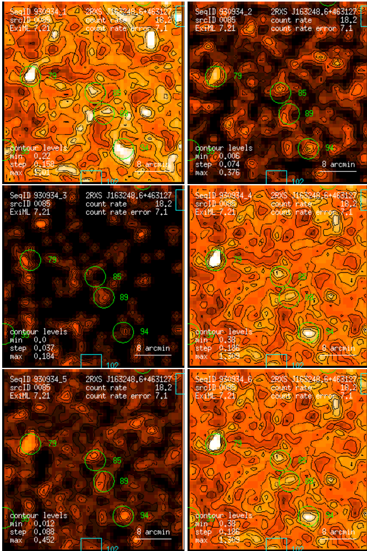
Figure 85: RASS 930934: detection 0085: band rate images, Gaussian filter: (1) PSPC channels 11 – 41, (2) 52 – 90, (3) 91 – 201, (4) 11 – 235, (5) 52 – 201, (6) 11 – 201. Broad band rates in counts/ks. Band rate contour levels in counts/ks/arcmin 2 .
