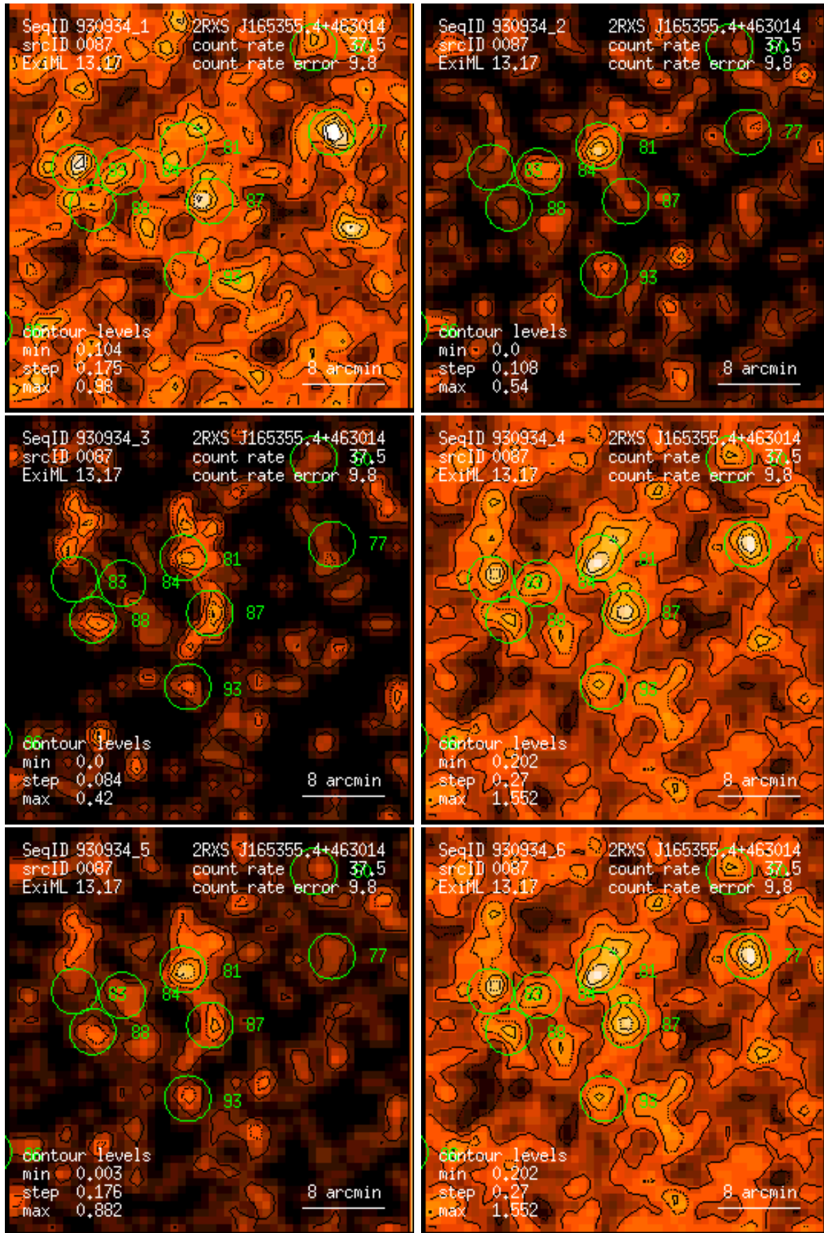
Figure 87: RASS 930934: detection 0087: band rate images, Gaussian filter: (1) PSPC channels 11 – 41, (2) 52 – 90, (3) 91 – 201, (4) 11 – 235, (5) 52 – 201, (6) 11 – 201. Broad band rates in counts/ks. Band rate contour levels in counts/ks/arcmin 2 .
