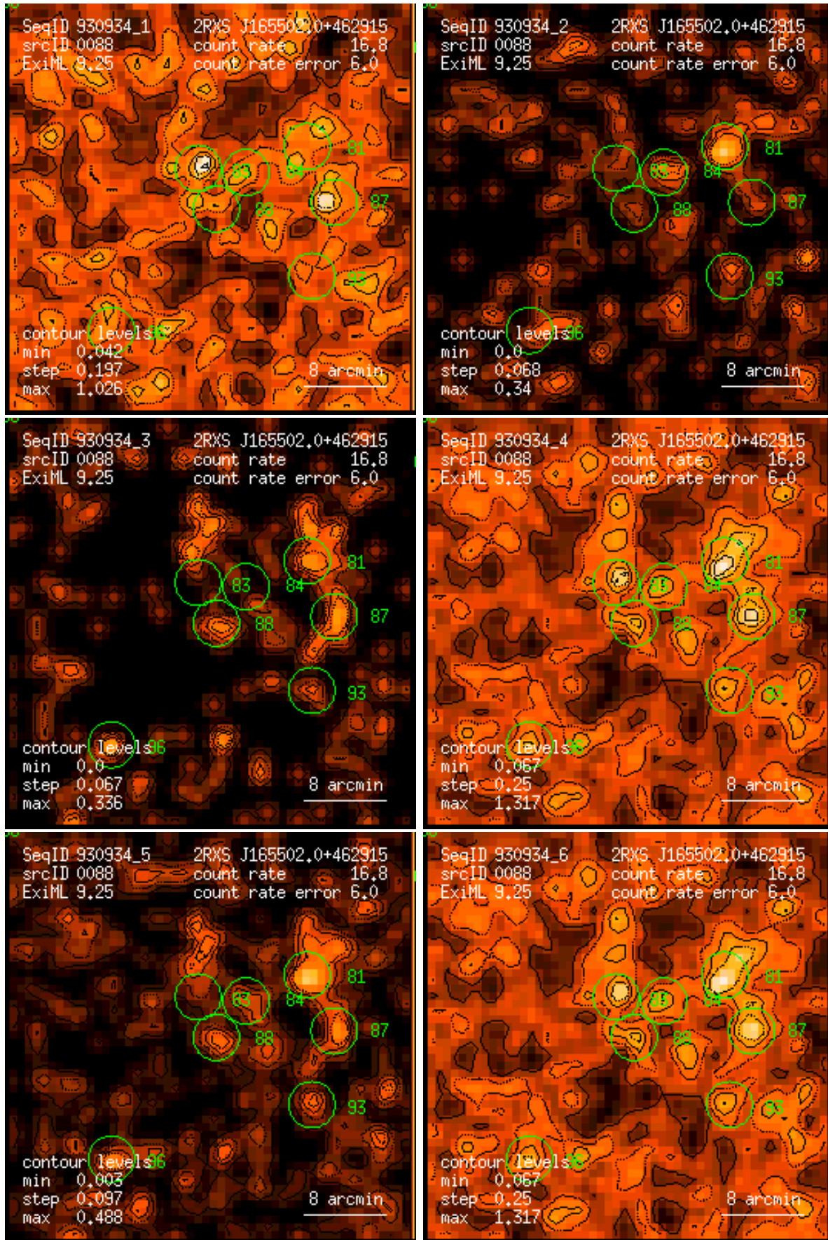
Figure 88: RASS 930934: detection 0088: band rate images, Gaussian filter: (1) PSPC channels 11 – 41, (2) 52 – 90, (3) 91 – 201, (4) 11 – 235, (5) 52 – 201, (6) 11 – 201. Broad band rates in counts/ks. Band rate contour levels in counts/ks/arcmin 2 .
