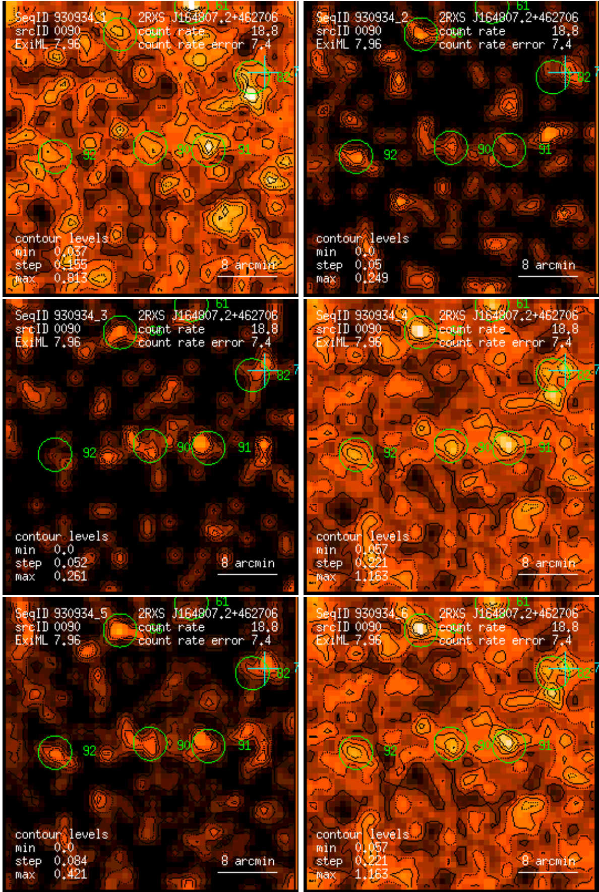
Figure 90: RASS 930934: detection 0090: band rate images, Gaussian filter: (1) PSPC channels 11 – 41, (2) 52 – 90, (3) 91 – 201, (4) 11 – 235, (5) 52 – 201, (6) 11 – 201. Broad band rates in counts/ks. Band rate contour levels in counts/ks/arcmin 2 .
