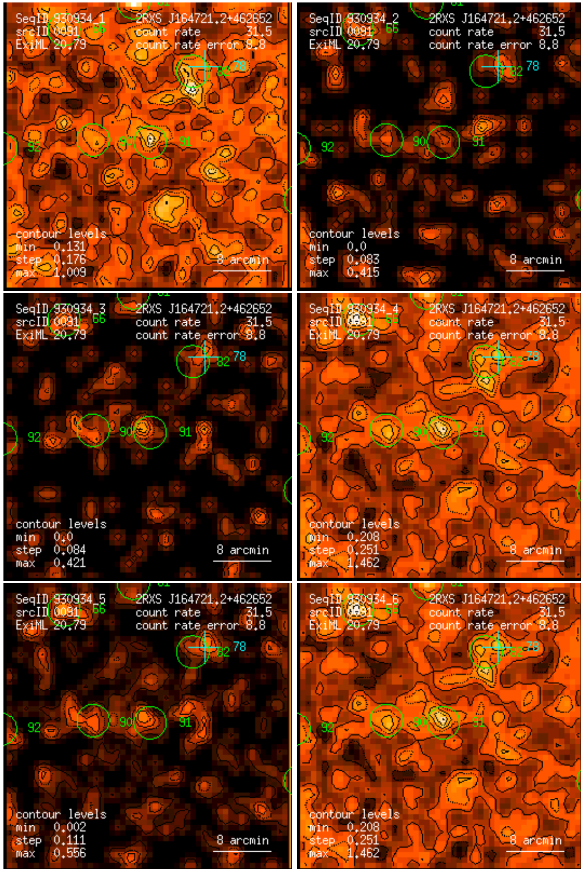
Figure 91: RASS 930934: detection 0091: band rate images, Gaussian filter: (1) PSPC channels 11 – 41, (2) 52 – 90, (3) 91 – 201, (4) 11 – 235, (5) 52 – 201, (6) 11 – 201. Broad band rates in counts/ks. Band rate contour levels in counts/ks/arcmin 2 .
