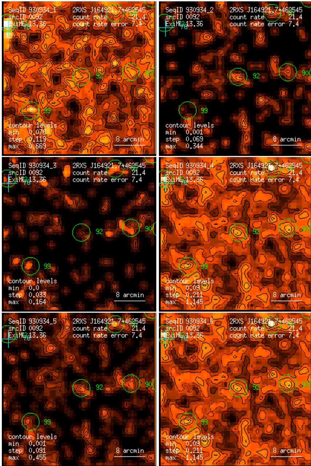
Figure 92: RASS 930934: detection 0092: band rate images, Gaussian filter: (1) PSPC channels 11 – 41, (2) 52 – 90, (3) 91 – 201, (4) 11 – 235, (5) 52 – 201, (6) 11 – 201. Broad band rates in counts/ks. Band rate contour levels in counts/ks/arcmin 2 .
