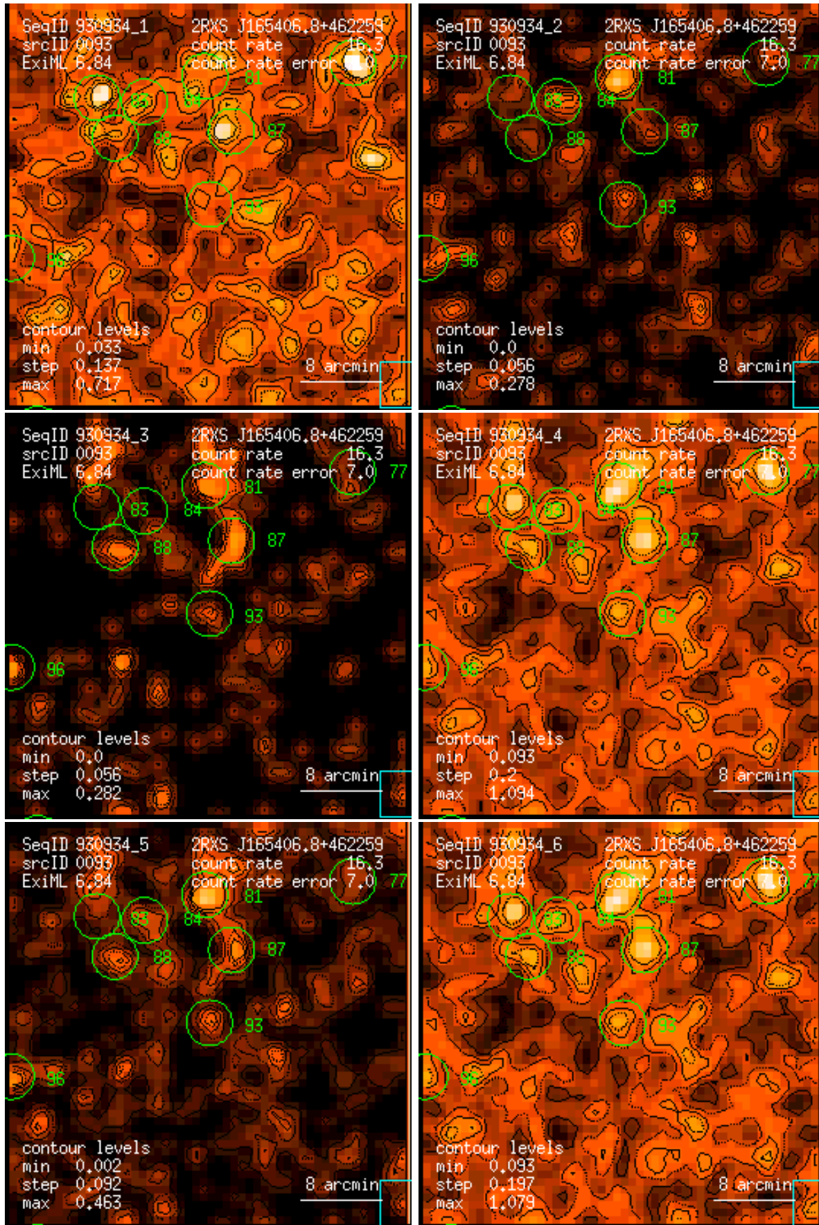
Figure 93: RASS 930934: detection 0093: band rate images, Gaussian filter: (1) PSPC channels 11 – 41, (2) 52 – 90, (3) 91 – 201, (4) 11 – 235, (5) 52 – 201, (6) 11 – 201. Broad band rates in counts/ks. Band rate contour levels in counts/ks/arcmin 2 .
