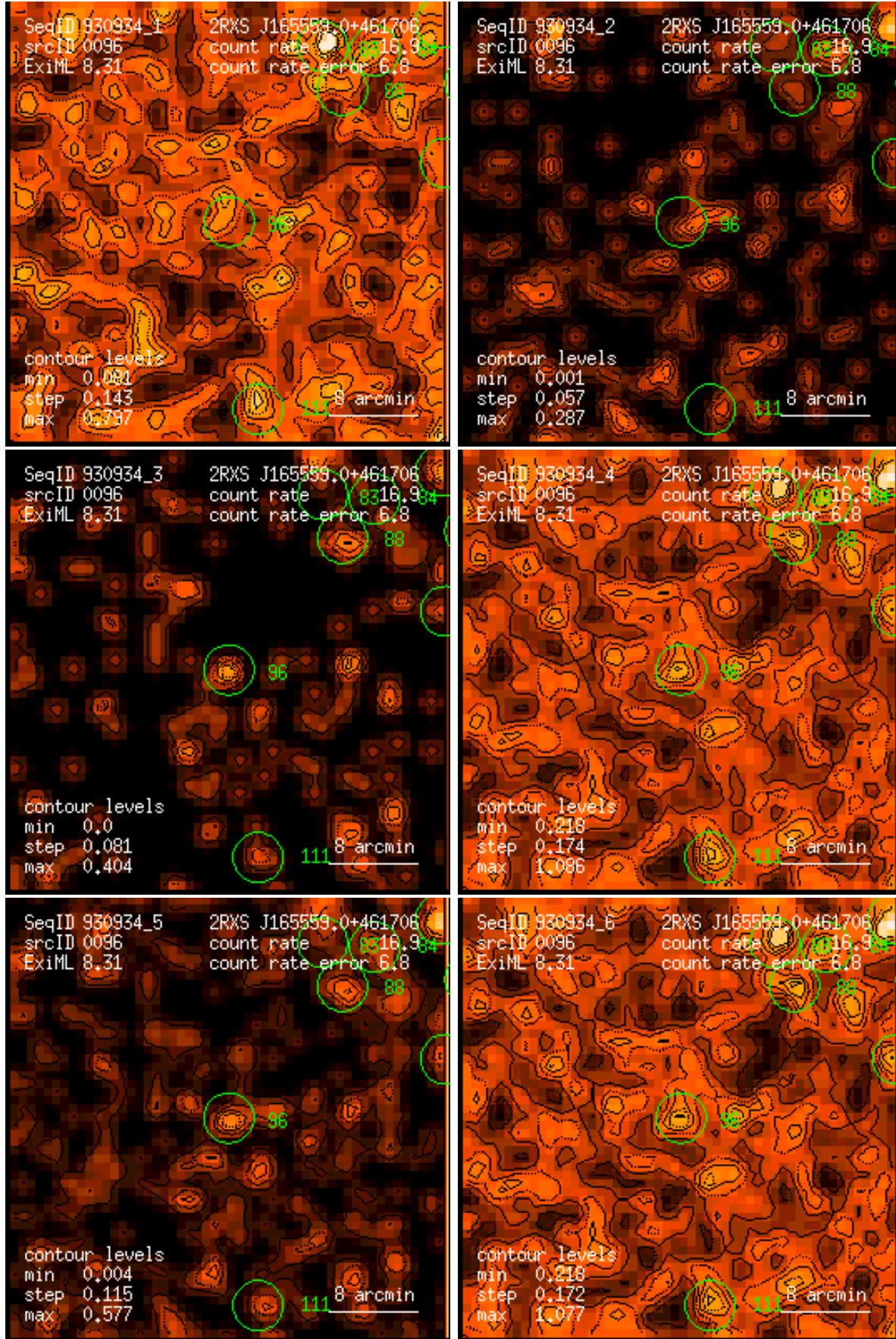
Figure 96: RASS 930934: detection 0096: band rate images, Gaussian filter: (1) PSPC channels 11 – 41, (2) 52 – 90, (3) 91 – 201, (4) 11 – 235, (5) 52 – 201, (6) 11 – 201. Broad band rates in counts/ks. Band rate contour levels in counts/ks/arcmin 2 .
