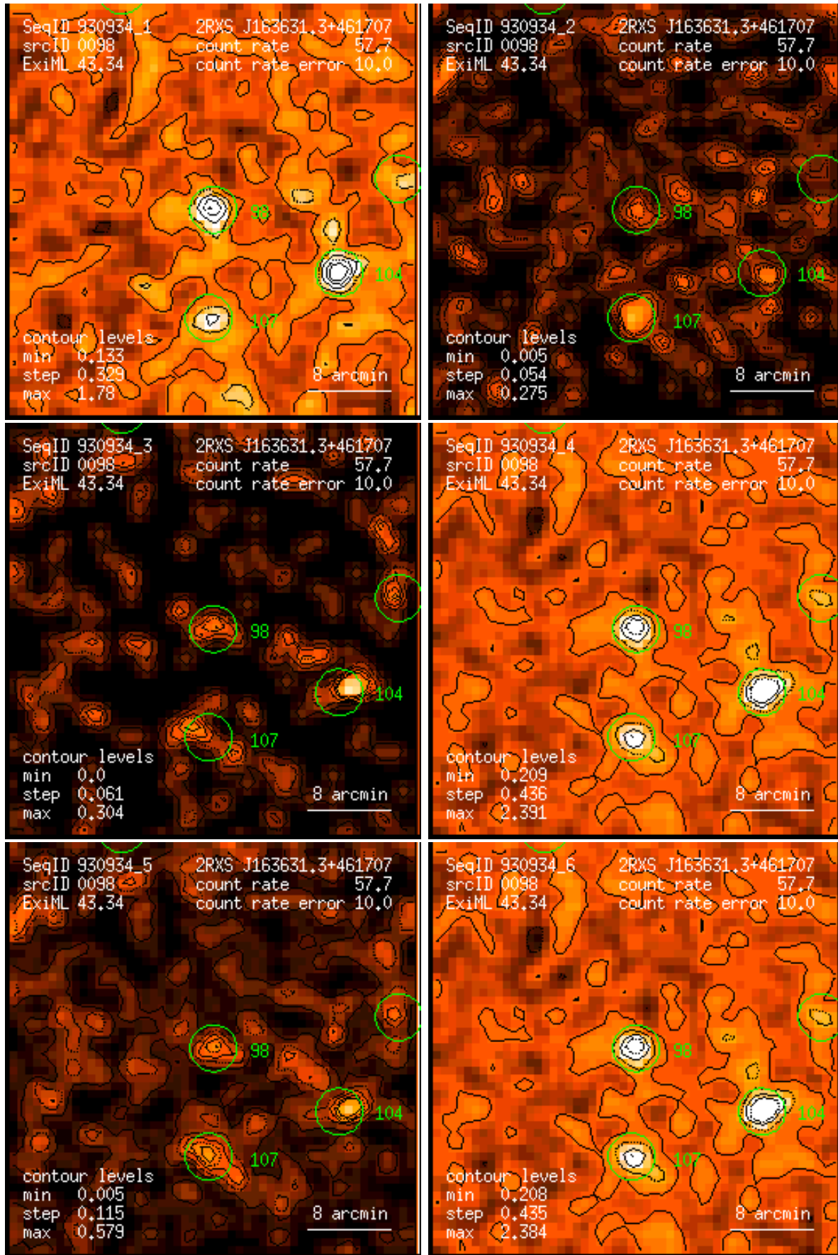
Figure 98: RASS 930934: detection 0098: band rate images, Gaussian filter: (1) PSPC channels 11 – 41, (2) 52 – 90, (3) 91 – 201, (4) 11 – 235, (5) 52 – 201, (6) 11 – 201. Broad band rates in counts/ks. Band rate contour levels in counts/ks/arcmin 2 .
