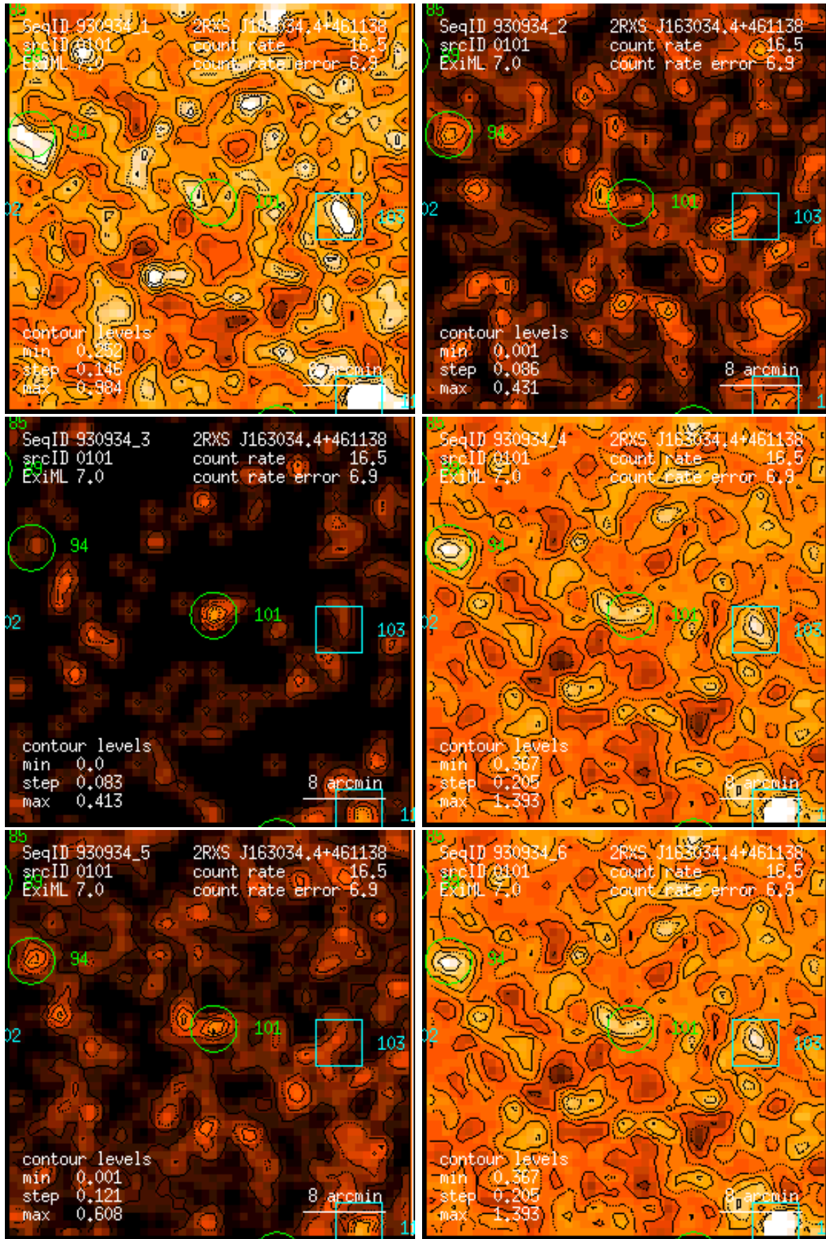
Figure 101: RASS 930934: detection 0101: band rate images, Gaussian filter: (1) PSPC channels 11 – 41, (2) 52 – 90, (3) 91 – 201, (4) 11 – 235, (5) 52 – 201, (6) 11 – 201. Broad band rates in counts/ks. Band rate contour levels in counts/ks/arcmin 2 .
