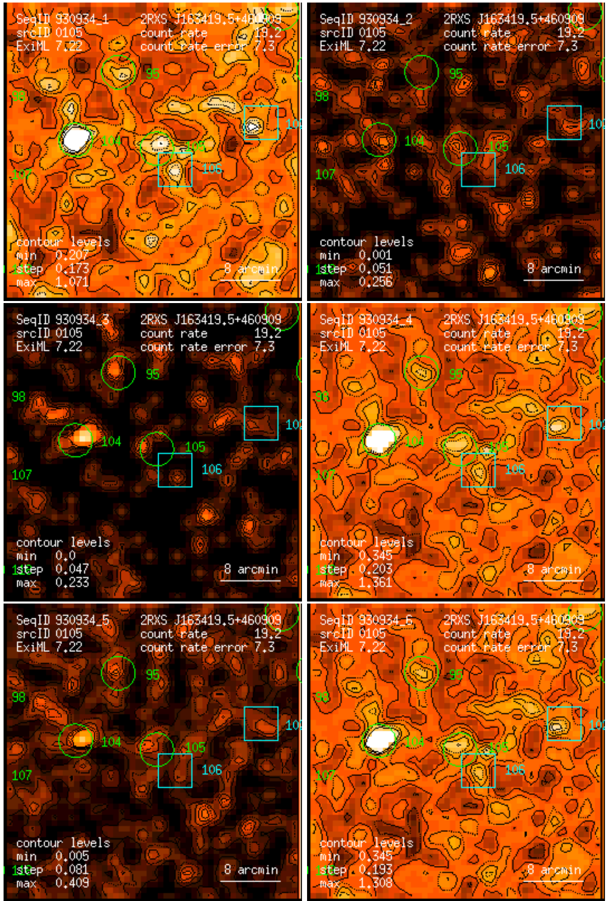
Figure 105: RASS 930934: detection 0105: band rate images, Gaussian filter: (1) PSPC channels 11 – 41, (2) 52 – 90, (3) 91 – 201, (4) 11 – 235, (5) 52 – 201, (6) 11 – 201. Broad band rates in counts/ks. Band rate contour levels in counts/ks/arcmin 2 .
