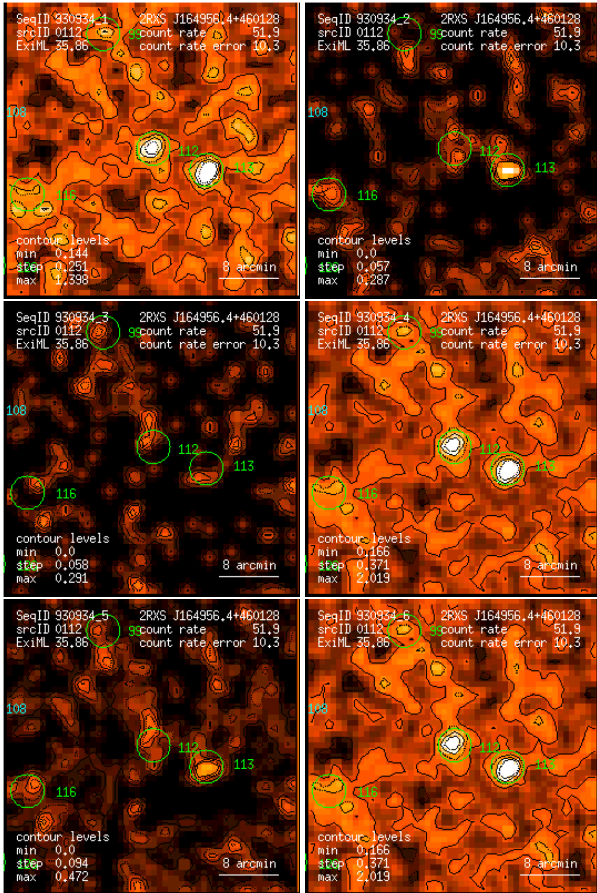
Figure 112: RASS 930934: detection 0112: band rate images, Gaussian filter: (1) PSPC channels 11 – 41, (2) 52 – 90, (3) 91 – 201, (4) 11 – 235, (5) 52 – 201, (6) 11 – 201. Broad band rates in counts/ks. Band rate contour levels in counts/ks/arcmin 2 .
