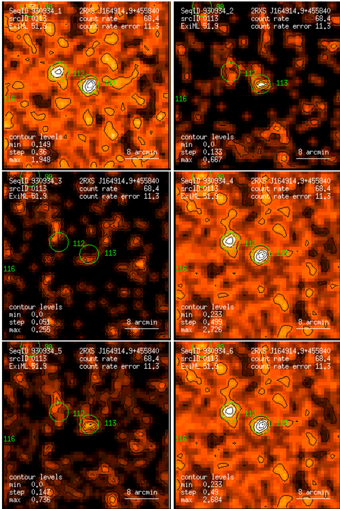
Figure 113: RASS 930934: detection 0113: band rate images, Gaussian filter: (1) PSPC channels 11 – 41, (2) 52 – 90, (3) 91 – 201, (4) 11 – 235, (5) 52 – 201, (6) 11 – 201. Broad band rates in counts/ks. Band rate contour levels in counts/ks/arcmin 2 .
