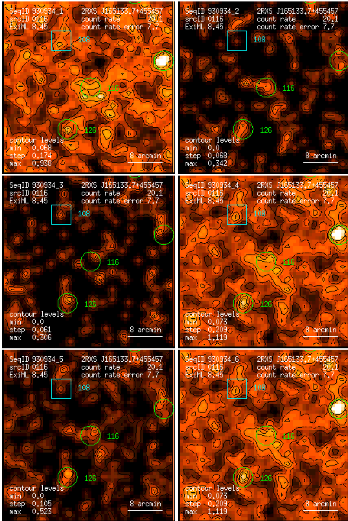
Figure 116: RASS 930934: detection 0116: band rate images, Gaussian filter: (1) PSPC channels 11 – 41, (2) 52 – 90, (3) 91 – 201, (4) 11 – 235, (5) 52 – 201, (6) 11 – 201. Broad band rates in counts/ks. Band rate contour levels in counts/ks/arcmin 2 .
