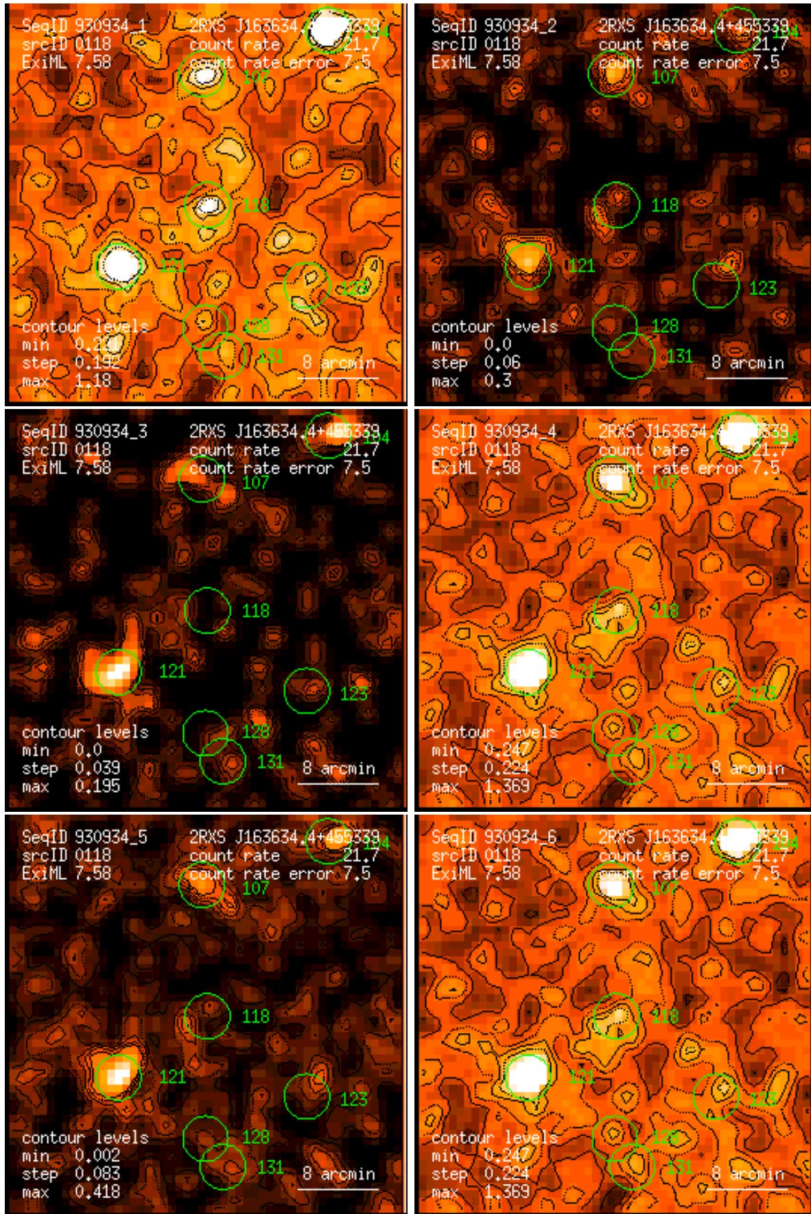
Figure 118: RASS 930934: detection 0118: band rate images, Gaussian filter: (1) PSPC channels 11 – 41, (2) 52 – 90, (3) 91 – 201, (4) 11 – 235, (5) 52 – 201, (6) 11 – 201. Broad band rates in counts/ks. Band rate contour levels in counts/ks/arcmin 2 .
