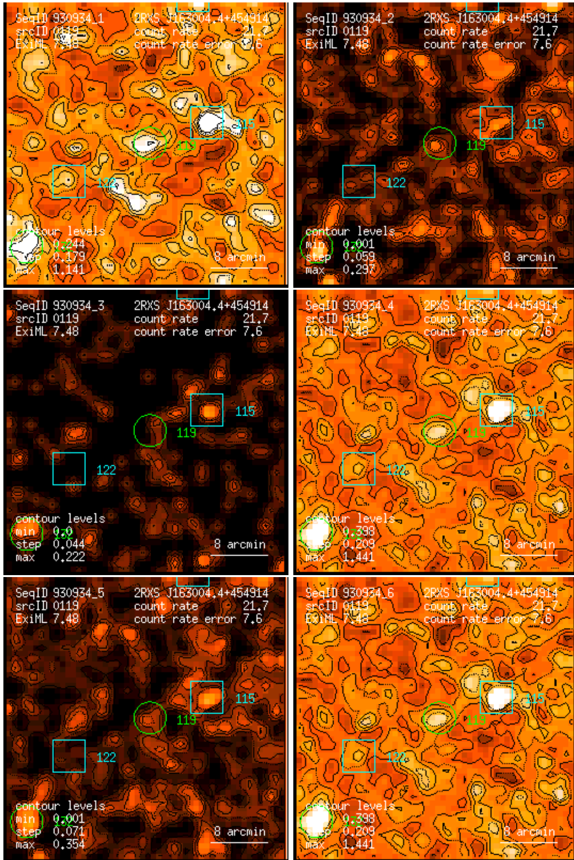
Figure 119: RASS 930934: detection 0119: band rate images, Gaussian filter: (1) PSPC channels 11 – 41, (2) 52 – 90, (3) 91 – 201, (4) 11 – 235, (5) 52 – 201, (6) 11 – 201. Broad band rates in counts/ks. Band rate contour levels in counts/ks/arcmin 2 .
