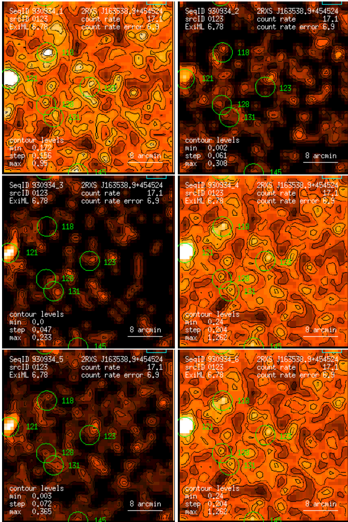
Figure 123: RASS 930934: detection 0123: band rate images, Gaussian filter: (1) PSPC channels 11 – 41, (2) 52 – 90, (3) 91 – 201, (4) 11 – 235, (5) 52 – 201, (6) 11 – 201. Broad band rates in counts/ks. Band rate contour levels in counts/ks/arcmin 2 .
