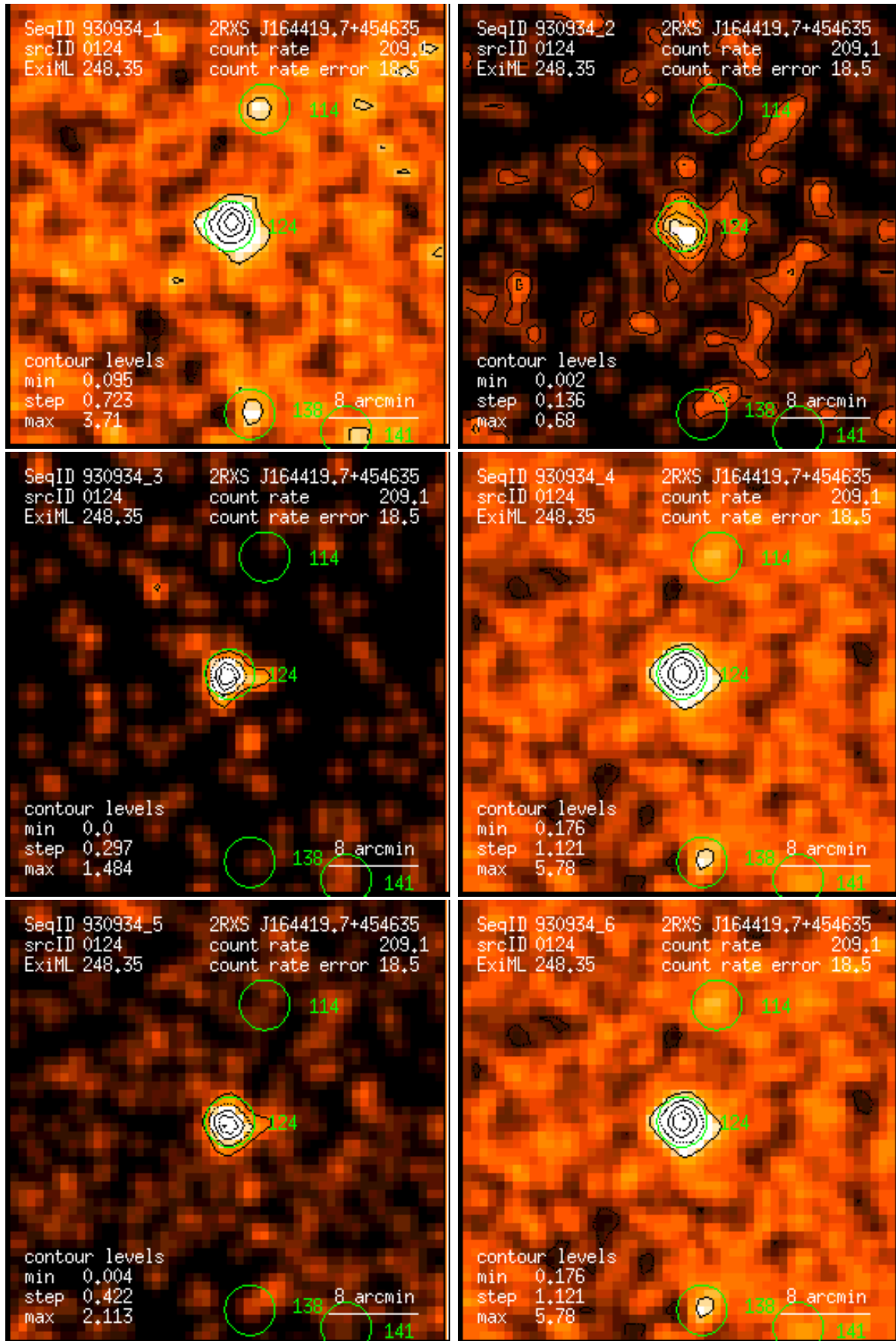
Figure 124: RASS 930934: detection 0124: band rate images, Gaussian filter: (1) PSPC channels 11 – 41, (2) 52 – 90, (3) 91 – 201, (4) 11 – 235, (5) 52 – 201, (6) 11 – 201. Broad band rates in counts/ks. Band rate contour levels in counts/ks/arcmin 2 .
