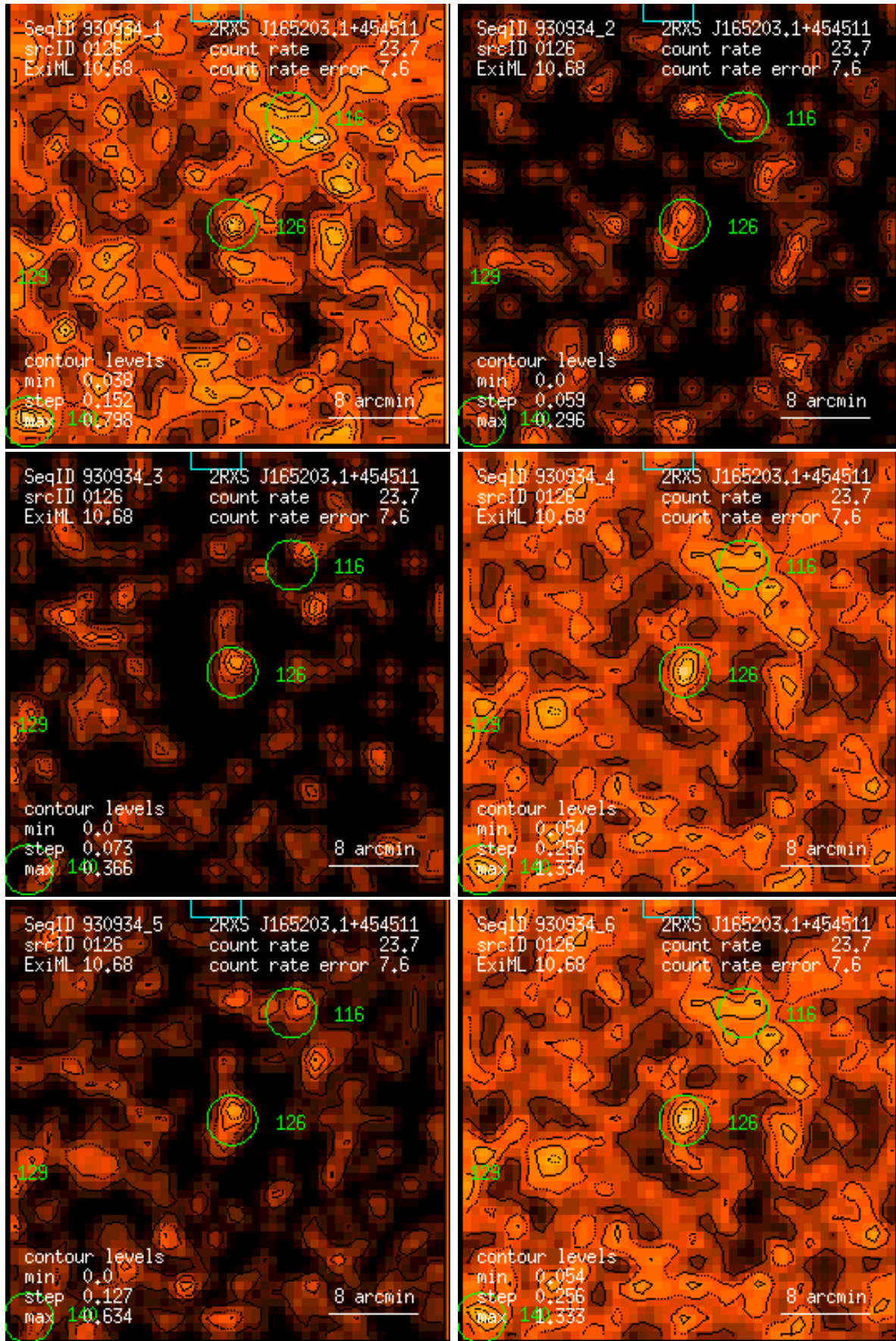
Figure 126: RASS 930934: detection 0126: band rate images, Gaussian filter: (1) PSPC channels 11 – 41, (2) 52 – 90, (3) 91 – 201, (4) 11 – 235, (5) 52 – 201, (6) 11 – 201. Broad band rates in counts/ks. Band rate contour levels in counts/ks/arcmin 2 .
