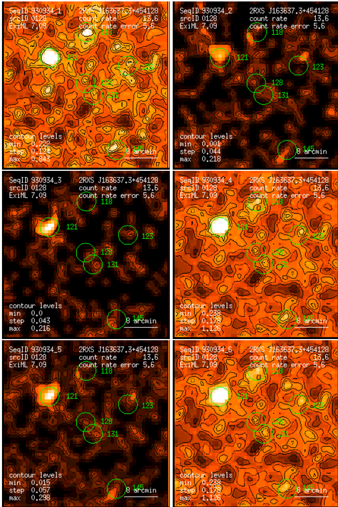
Figure 128: RASS 930934: detection 0128: band rate images, Gaussian filter: (1) PSPC channels 11 – 41, (2) 52 – 90, (3) 91 – 201, (4) 11 – 235, (5) 52 – 201, (6) 11 – 201. Broad band rates in counts/ks. Band rate contour levels in counts/ks/arcmin 2 .
