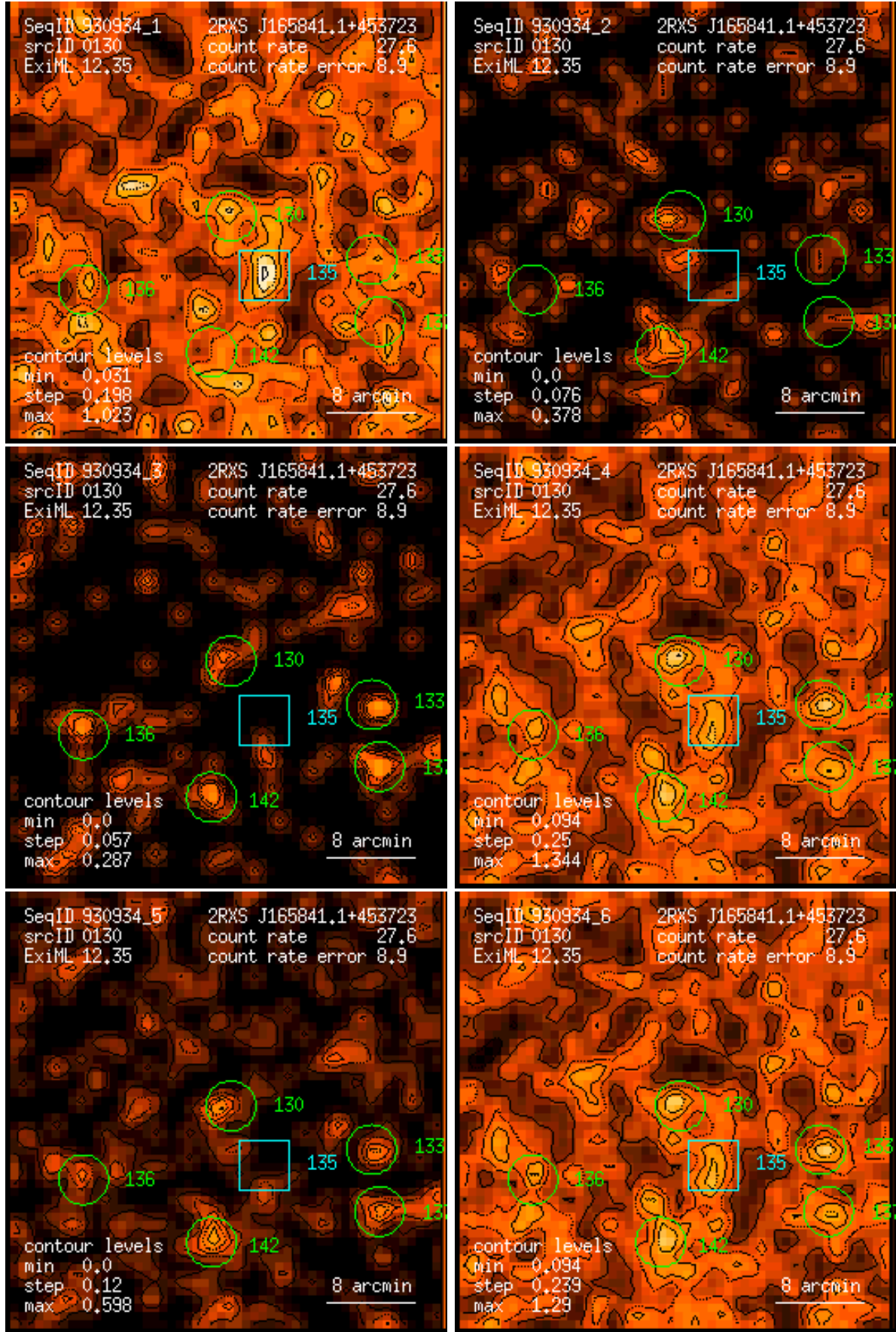
Figure 130: RASS 930934: detection 0130: band rate images, Gaussian filter: (1) PSPC channels 11 – 41, (2) 52 – 90, (3) 91 – 201, (4) 11 – 235, (5) 52 – 201, (6) 11 – 201. Broad band rates in counts/ks. Band rate contour levels in counts/ks/arcmin 2 .
