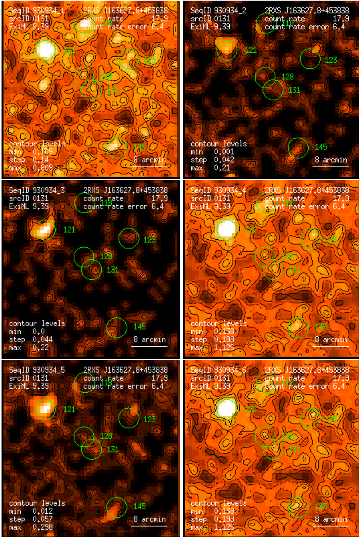
Figure 131: RASS 930934: detection 0131: band rate images, Gaussian filter: (1) PSPC channels 11 – 41, (2) 52 – 90, (3) 91 – 201, (4) 11 – 235, (5) 52 – 201, (6) 11 – 201. Broad band rates in counts/ks. Band rate contour levels in counts/ks/arcmin 2 .
