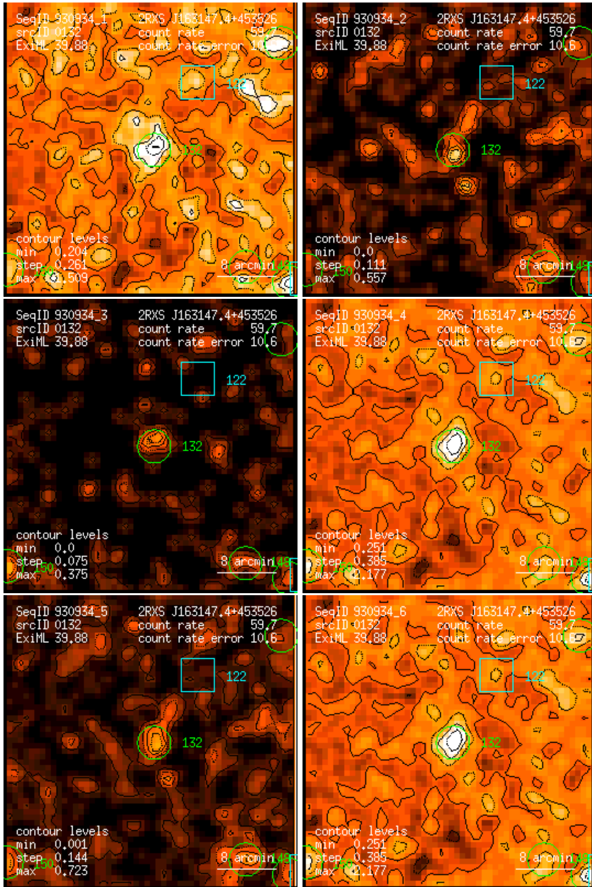
Figure 132: RASS 930934: detection 0132: band rate images, Gaussian filter: (1) PSPC channels 11 – 41, (2) 52 – 90, (3) 91 – 201, (4) 11 – 235, (5) 52 – 201, (6) 11 – 201. Broad band rates in counts/ks. Band rate contour levels in counts/ks/arcmin 2 .
