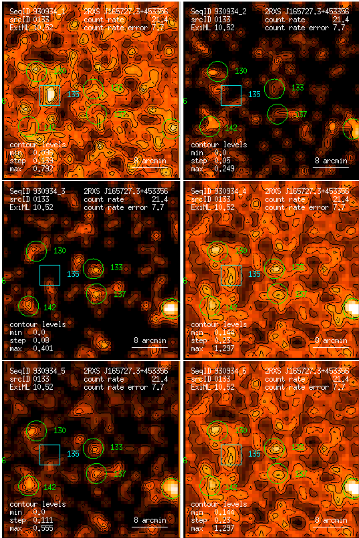
Figure 133: RASS 930934: detection 0133: band rate images, Gaussian filter: (1) PSPC channels 11 – 41, (2) 52 – 90, (3) 91 – 201, (4) 11 – 235, (5) 52 – 201, (6) 11 – 201. Broad band rates in counts/ks. Band rate contour levels in counts/ks/arcmin 2 .
