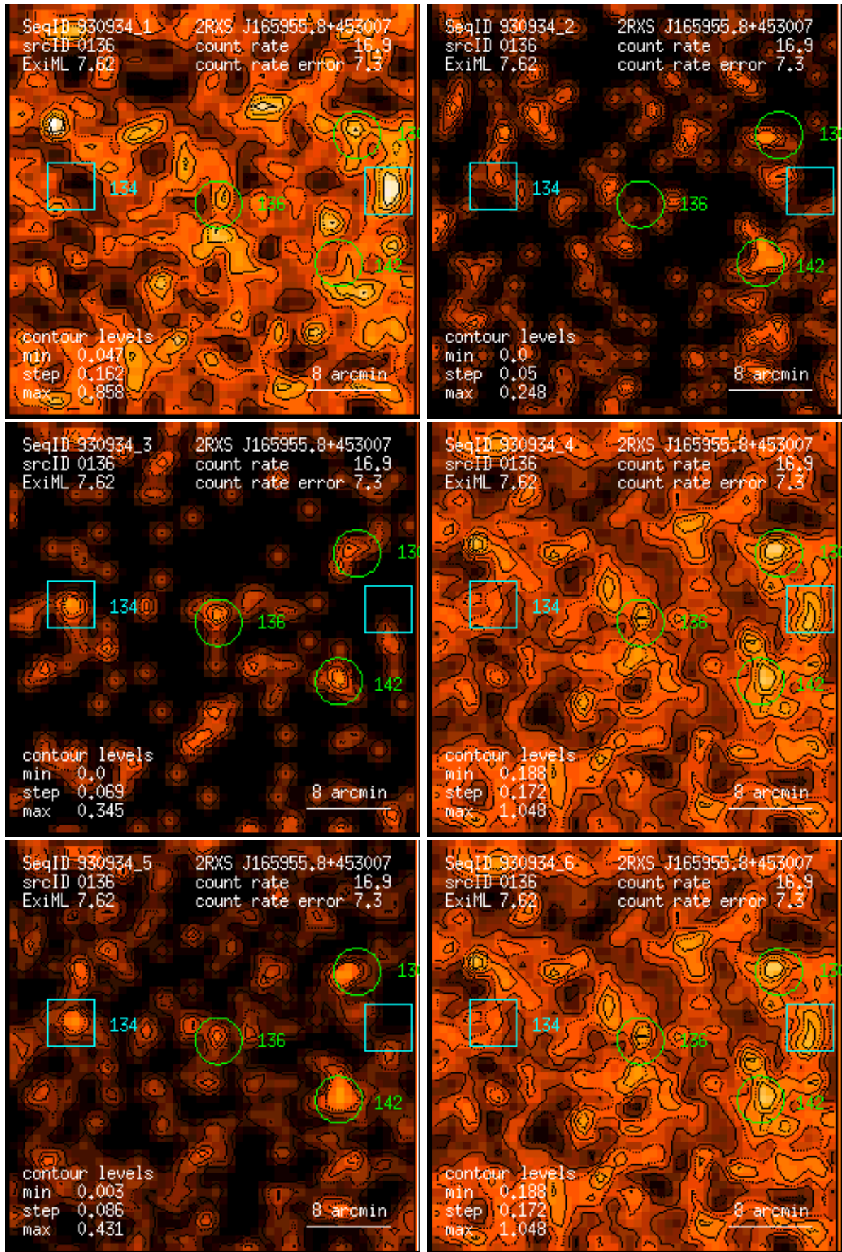
Figure 136: RASS 930934: detection 0136: band rate images, Gaussian filter: (1) PSPC channels 11 – 41, (2) 52 – 90, (3) 91 – 201, (4) 11 – 235, (5) 52 – 201, (6) 11 – 201. Broad band rates in counts/ks. Band rate contour levels in counts/ks/arcmin 2 .
