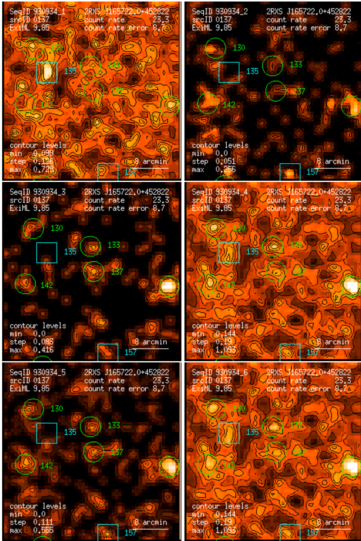
Figure 137: RASS 930934: detection 0137: band rate images, Gaussian filter: (1) PSPC channels 11 – 41, (2) 52 – 90, (3) 91 – 201, (4) 11 – 235, (5) 52 – 201, (6) 11 – 201. Broad band rates in counts/ks. Band rate contour levels in counts/ks/arcmin 2 .
