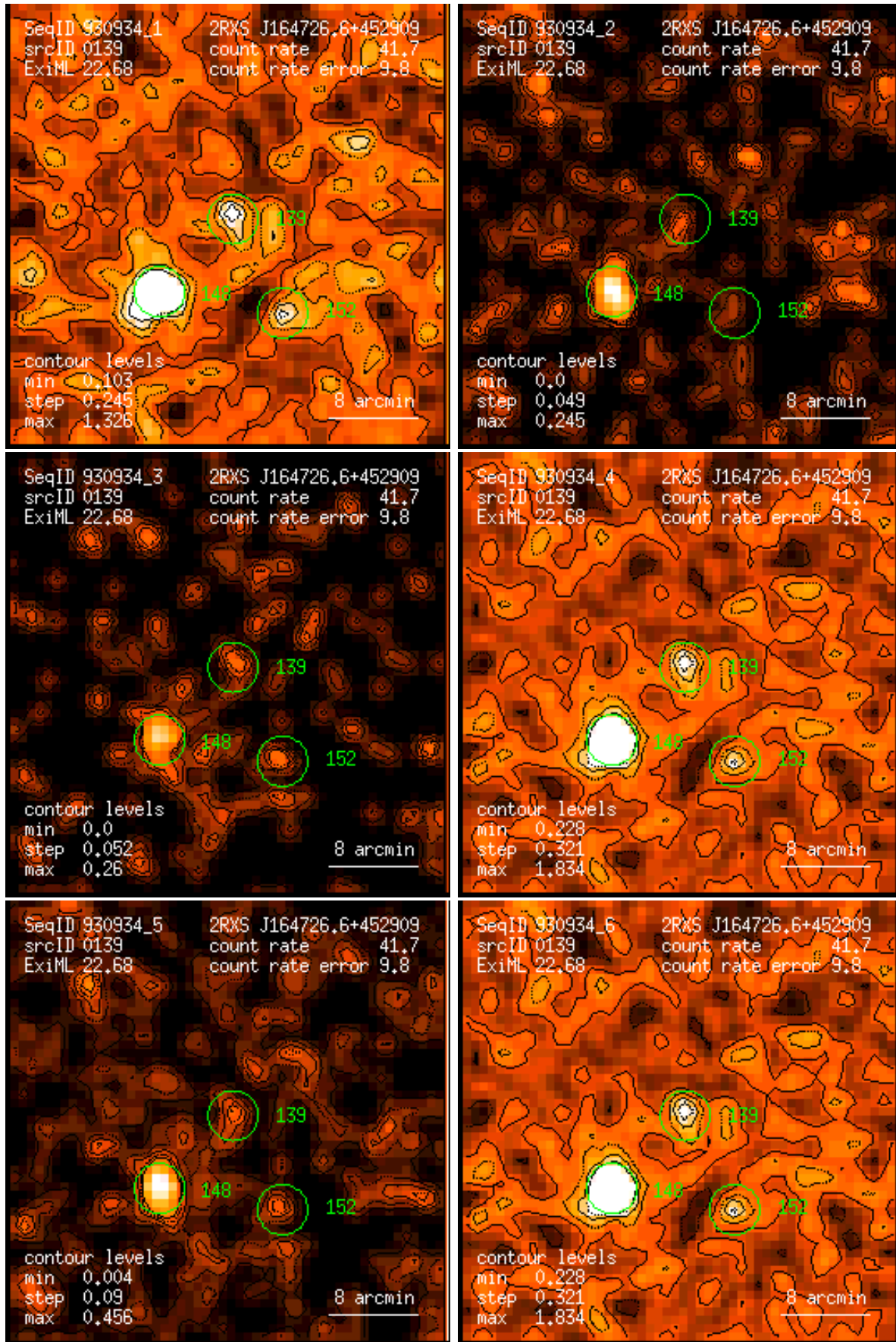
Figure 139: RASS 930934: detection 0139: band rate images, Gaussian filter: (1) PSPC channels 11 – 41, (2) 52 – 90, (3) 91 – 201, (4) 11 – 235, (5) 52 – 201, (6) 11 – 201. Broad band rates in counts/ks. Band rate contour levels in counts/ks/arcmin 2 .
