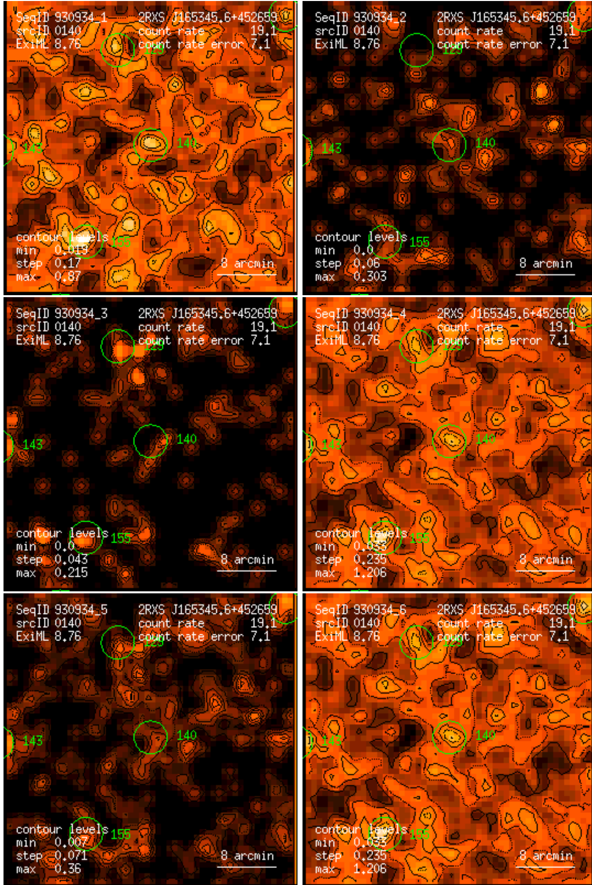
Figure 140: RASS 930934: detection 0140: band rate images, Gaussian filter: (1) PSPC channels 11 – 41, (2) 52 – 90, (3) 91 – 201, (4) 11 – 235, (5) 52 – 201, (6) 11 – 201. Broad band rates in counts/ks. Band rate contour levels in counts/ks/arcmin 2 .
