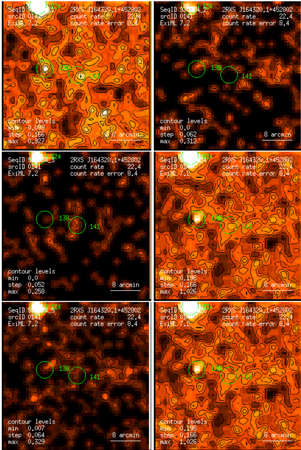
Figure 141: RASS 930934: detection 0141: band rate images, Gaussian filter: (1) PSPC channels 11 – 41, (2) 52 – 90, (3) 91 – 201, (4) 11 – 235, (5) 52 – 201, (6) 11 – 201. Broad band rates in counts/ks. Band rate contour levels in counts/ks/arcmin 2 .
