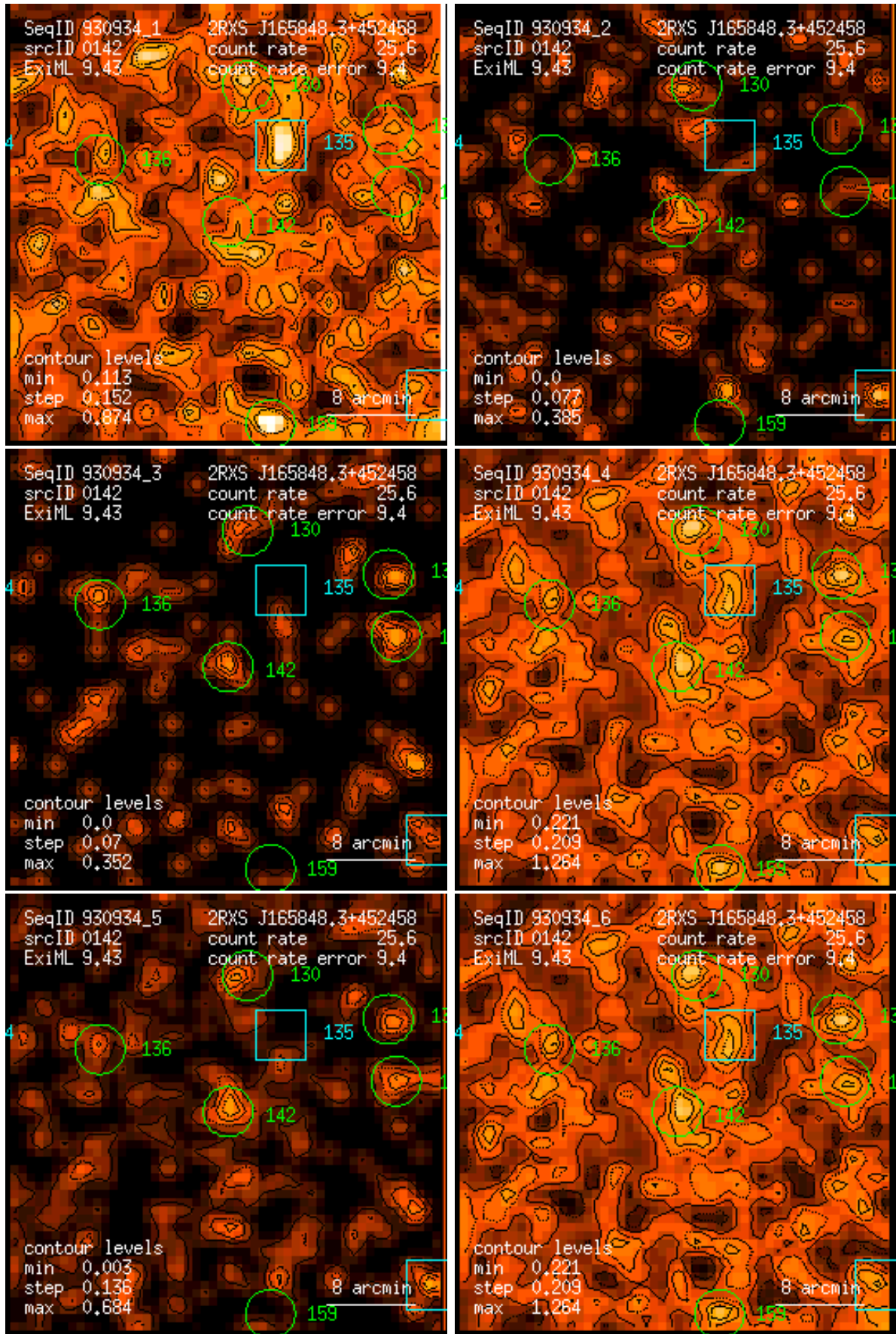
Figure 142: RASS 930934: detection 0142: band rate images, Gaussian filter: (1) PSPC channels 11 – 41, (2) 52 – 90, (3) 91 – 201, (4) 11 – 235, (5) 52 – 201, (6) 11 – 201. Broad band rates in counts/ks. Band rate contour levels in counts/ks/arcmin 2 .
