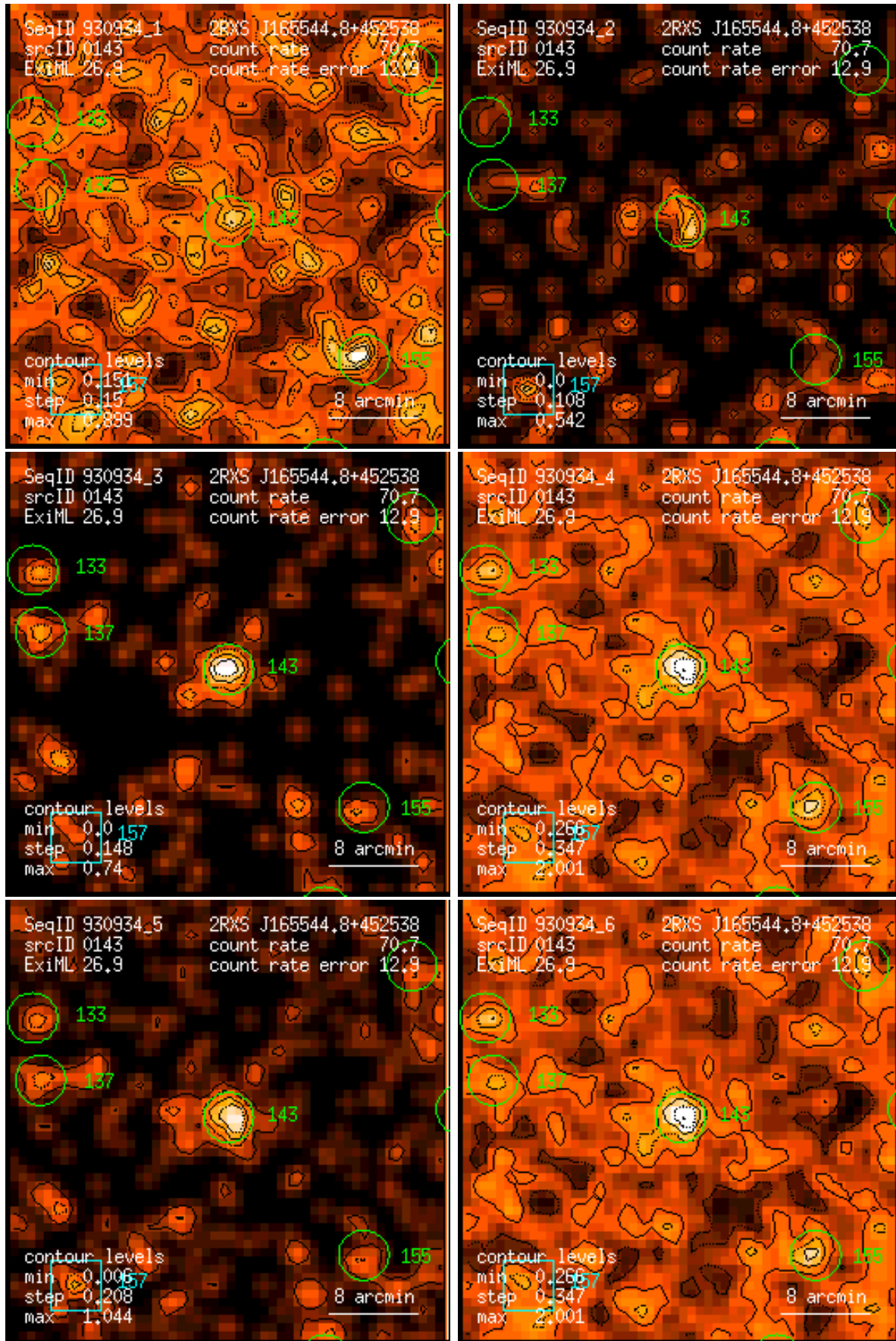
Figure 143: RASS 930934: detection 0143: band rate images, Gaussian filter: (1) PSPC channels 11 – 41, (2) 52 – 90, (3) 91 – 201, (4) 11 – 235, (5) 52 – 201, (6) 11 – 201. Broad band rates in counts/ks. Band rate contour levels in counts/ks/arcmin 2 .
