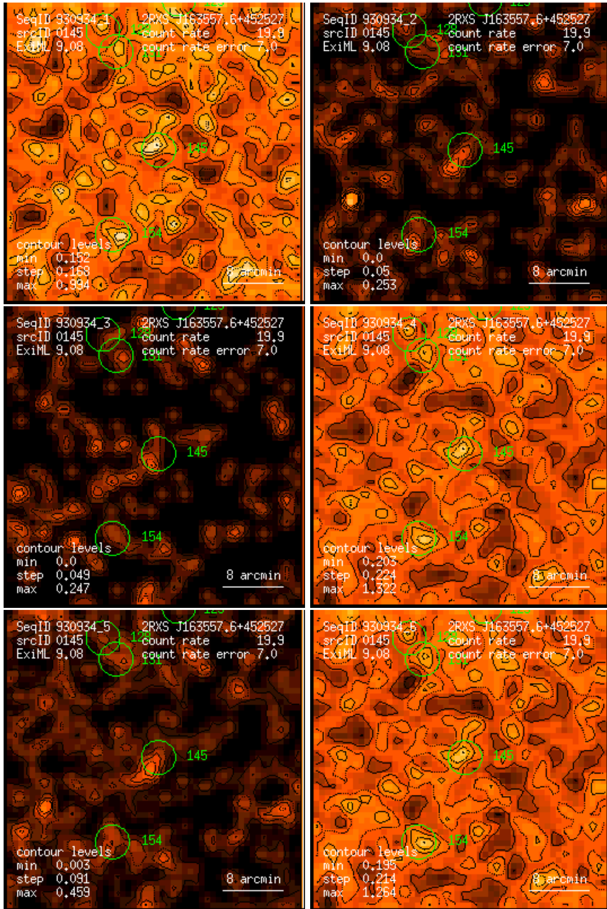
Figure 145: RASS 930934: detection 0145: band rate images, Gaussian filter: (1) PSPC channels 11 – 41, (2) 52 – 90, (3) 91 – 201, (4) 11 – 235, (5) 52 – 201, (6) 11 – 201. Broad band rates in counts/ks. Band rate contour levels in counts/ks/arcmin 2 .
