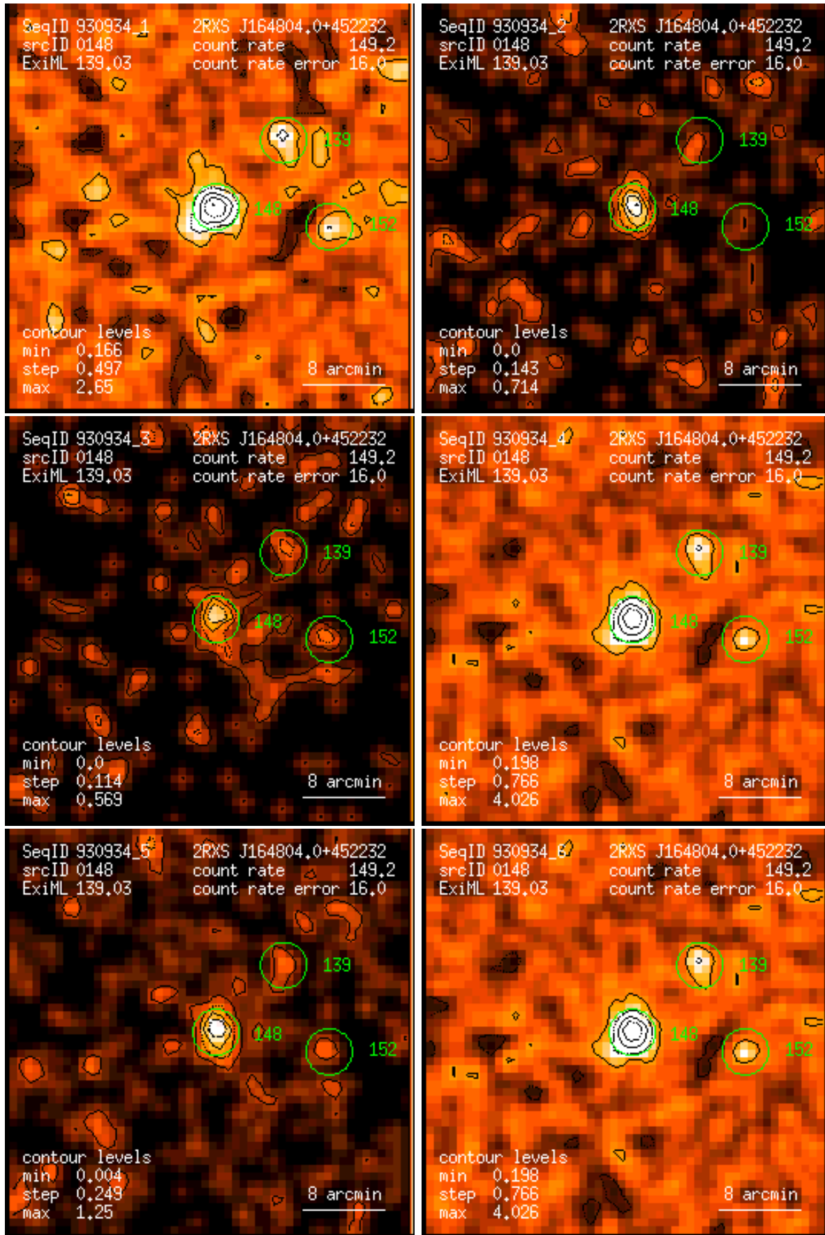
Figure 148: RASS 930934: detection 0148: band rate images, Gaussian filter: (1) PSPC channels 11 – 41, (2) 52 – 90, (3) 91 – 201, (4) 11 – 235, (5) 52 – 201, (6) 11 – 201. Broad band rates in counts/ks. Band rate contour levels in counts/ks/arcmin 2 .
