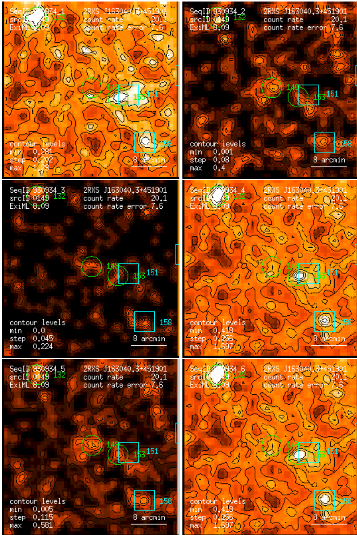
Figure 149: RASS 930934: detection 0149: band rate images, Gaussian filter: (1) PSPC channels 11 – 41, (2) 52 – 90, (3) 91 – 201, (4) 11 – 235, (5) 52 – 201, (6) 11 – 201. Broad band rates in counts/ks. Band rate contour levels in counts/ks/arcmin 2 .
