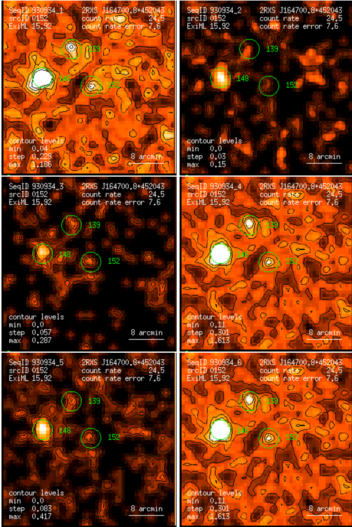
Figure 152: RASS 930934: detection 0152: band rate images, Gaussian filter: (1) PSPC channels 11 – 41, (2) 52 – 90, (3) 91 – 201, (4) 11 – 235, (5) 52 – 201, (6) 11 – 201. Broad band rates in counts/ks. Band rate contour levels in counts/ks/arcmin 2 .
