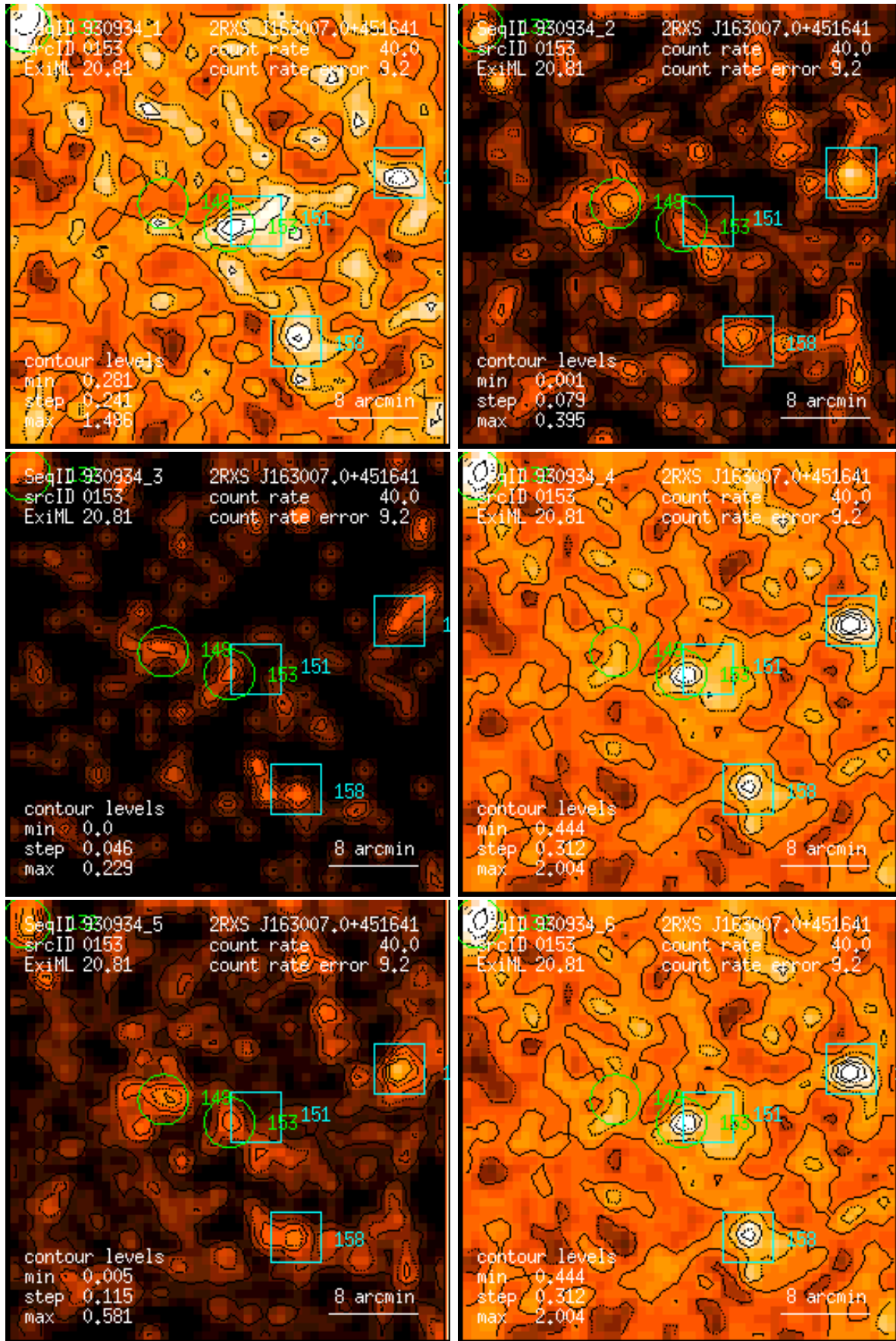
Figure 153: RASS 930934: detection 0153: band rate images, Gaussian filter: (1) PSPC channels 11 – 41, (2) 52 – 90, (3) 91 – 201, (4) 11 – 235, (5) 52 – 201, (6) 11 – 201. Broad band rates in counts/ks. Band rate contour levels in counts/ks/arcmin 2 .
