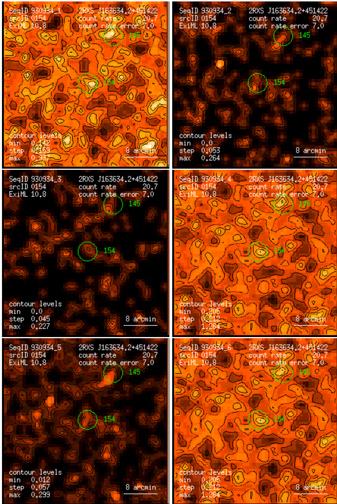
Figure 154: RASS 930934: detection 0154: band rate images, Gaussian filter: (1) PSPC channels 11 – 41, (2) 52 – 90, (3) 91 – 201, (4) 11 – 235, (5) 52 – 201, (6) 11 – 201. Broad band rates in counts/ks. Band rate contour levels in counts/ks/arcmin 2 .
