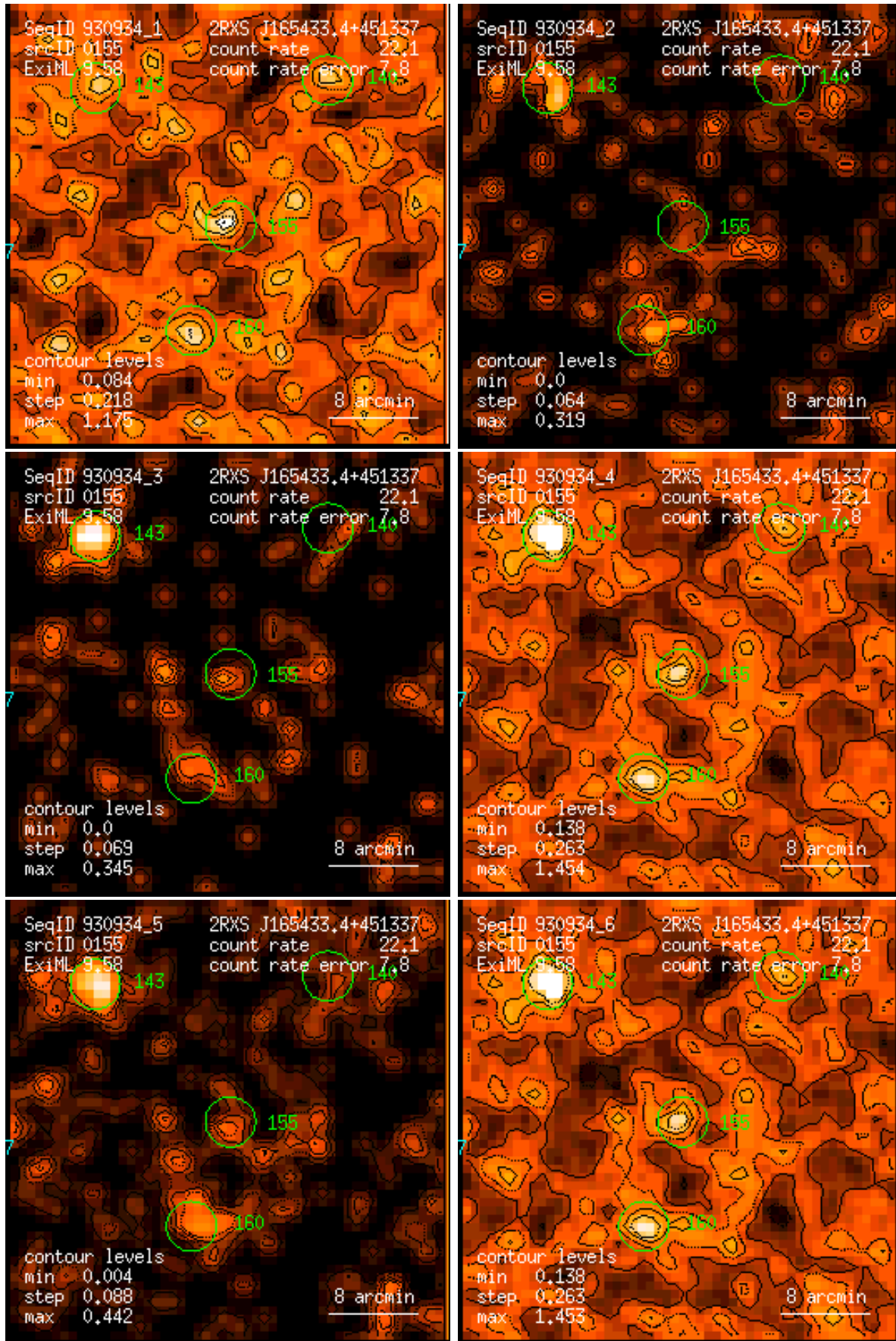
Figure 155: RASS 930934: detection 0155: band rate images, Gaussian filter: (1) PSPC channels 11 – 41, (2) 52 – 90, (3) 91 – 201, (4) 11 – 235, (5) 52 – 201, (6) 11 – 201. Broad band rates in counts/ks. Band rate contour levels in counts/ks/arcmin 2 .
